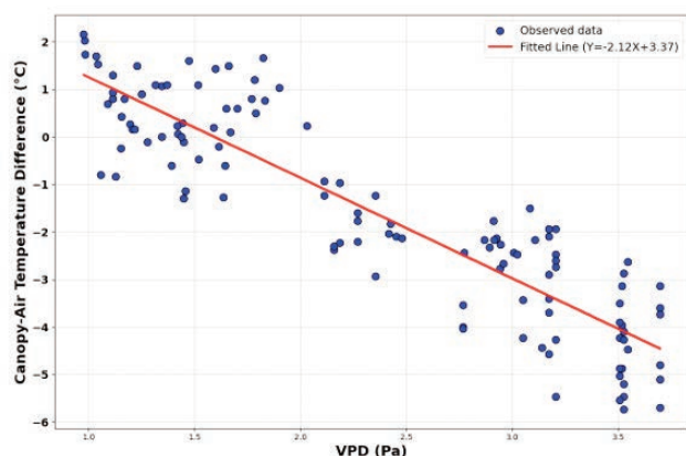
Figure 5. Linear regression relationship between VPD and the lower bound of the canopy-air temperature difference ( T_c - T_a ) under fully irrigated conditions. The fitted line ( Y = -2.12X + 3.37 ) demonstrates a strong negative correlation ( R^2=0.811 ), confirming the importance of VPD as an indicator of water stress in tea trees.
