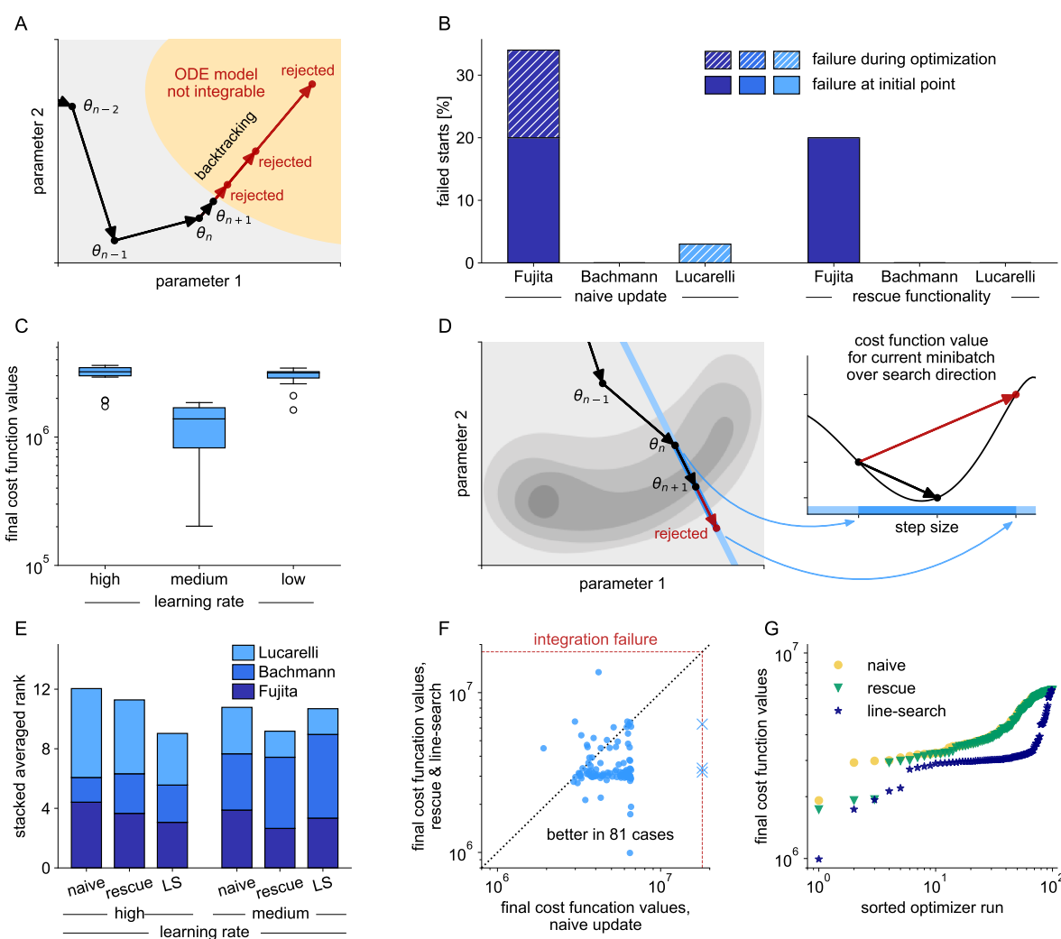
Figure 3: Influence of line-search methods on optimizers performance and reliability. A Schematic of the rescue functionality, which tries to recover from failed model evaluations, based on backtracking line-search. B Percentage of failed local optimizations per model (with optimizer Adam) due to non-integrability of the underlying ODE. Failure at the initial point of optimization can not be recovered, but failure during the optimization process is prevented when applying the rescue functionality. C Boxplots for the best 25 starts of mini-batch optimizers Adam for three different learning rates for the largest example (Lucarelli), showing that too high learning rates obstruct the optimization process. D Line-search implementation for mini-batch optimizers is implemented based on backtracking, while keeping the mini-batch fixed during line-search. E Comparison of performance for optimizer Adam, given different learning rates, for naive implementation, with rescue functionality, and rescue functionality and line-search (ranks of models are stacked). F All starts of the local optimizer Adam for the largest of the three examples (Lucarelli), naive implementation compared against rescue functionality and line-search, employing a high learning rate. G Waterfall plot for the largest of the three examples (Lucarelli), for naive implementation of Adam, with rescue functionality and with rescue functionality and line-search.
