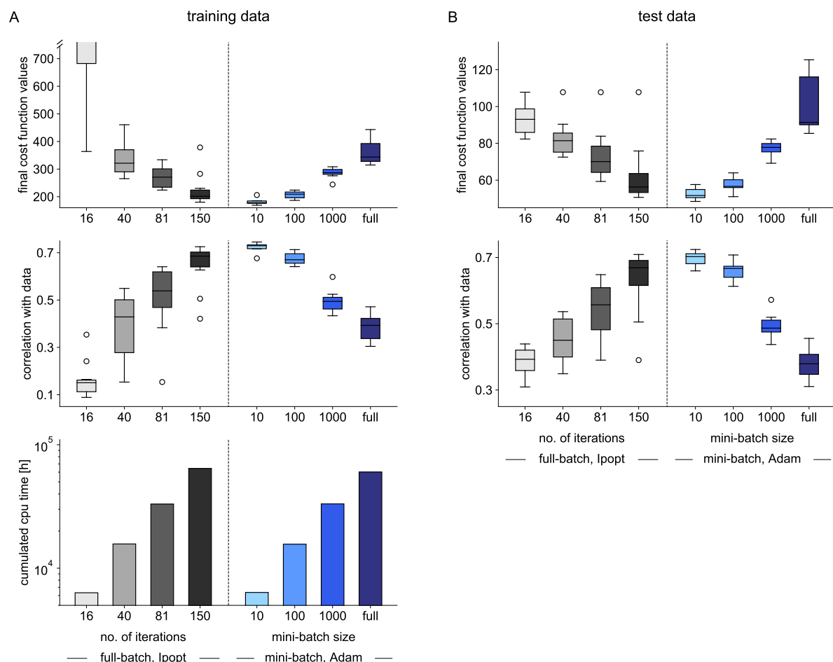
Figure 6: Comparison of optimization results for the large-scale cancer model, for different mini-batch sizes at low learning rate. A Boxplots of the 10 best optimization runs out of 20, started at the same random parameters, for Ipopt (at four different stages of the optimization process to compare performance over computation time) and for mini-batch optimization with different optimization settings on training data: final objective functions values (upper panel), correlation of model simulation with measurement data (middle panel), and total computation time for all 20 optimization runs (lower panel). B Evaluation of objective function values and correlation with measurement data for results from A on independent test data.
