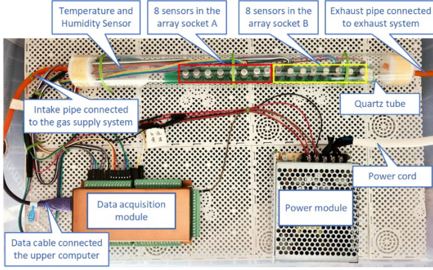
Fig. 5 Experimental setup used for data acquisition.
