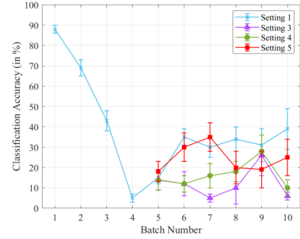
Fig. 3 The performance of the classifiers obtained from Setting 1 (x), Setting 3 (Δ), Setting 4 (○), and Setting 5 (□) is depicted in the graph. The red continuous line represents the results achieved using Setting 5 (□), which is the proposed method in this paper.
