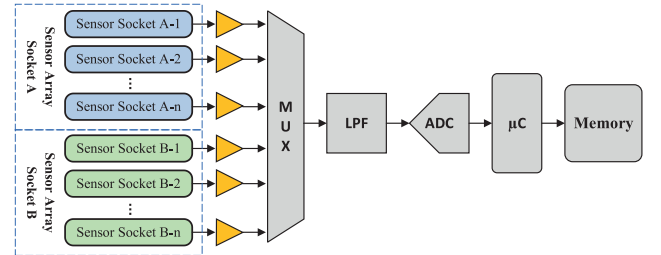
Fig. 1 Sensor arrays with interface electronics blocks, which include the amplifiers, multiplexer (MUX), low-pass filter (LPF), analog to digital converter (ADC), microcontroller ( \mu C ) and memory.
