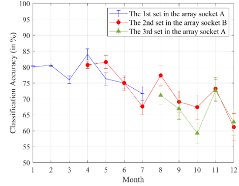
Fig. 6 The classification performance of the original sensor array and that after two sensor replacements.
