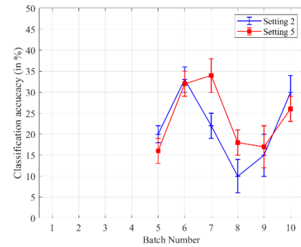
Fig. 4 The classifier performance comparison between the traditional method (Setting 2 (+)) and the proposed method in this paper (Setting 5 (□)) is shown in the graph.
