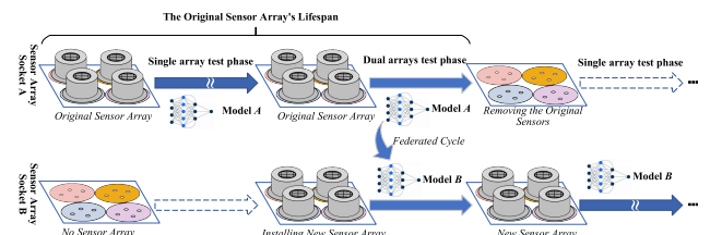
Fig. 2 Overview of the FedGSSU method.
