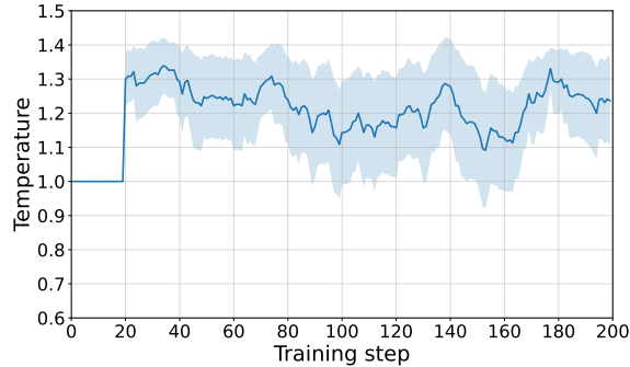
Figure 3: Sampling temperatures from the meta-policy using nucleus sampling.
