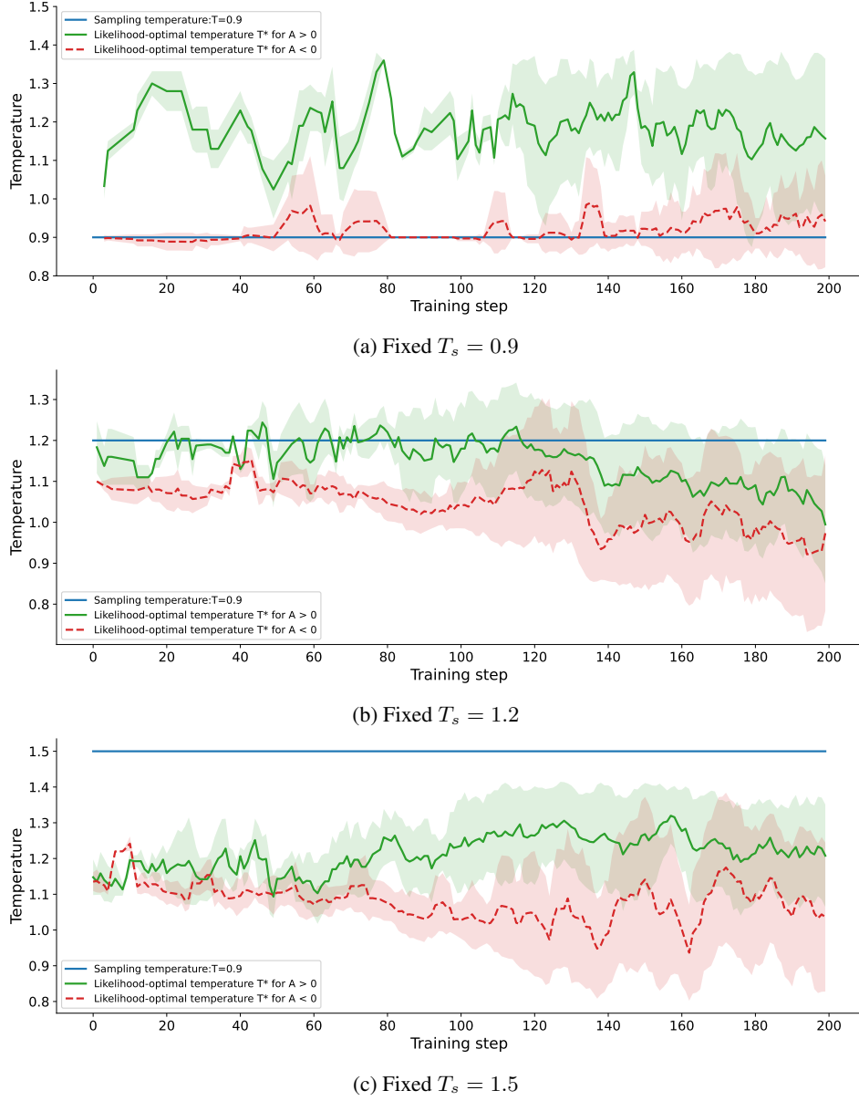
Figure 4: Distribution of trajectory likelihood-optimal temperatures under three fixed training temperatures, respectively. Green curve corresponds to the likelihood-optimal temperatures of positive-advantage trajectories ( A > 0 ), red curve to negative-advantage trajectories ( A < 0 ), and blue curve to the sampled fixed temperature.
