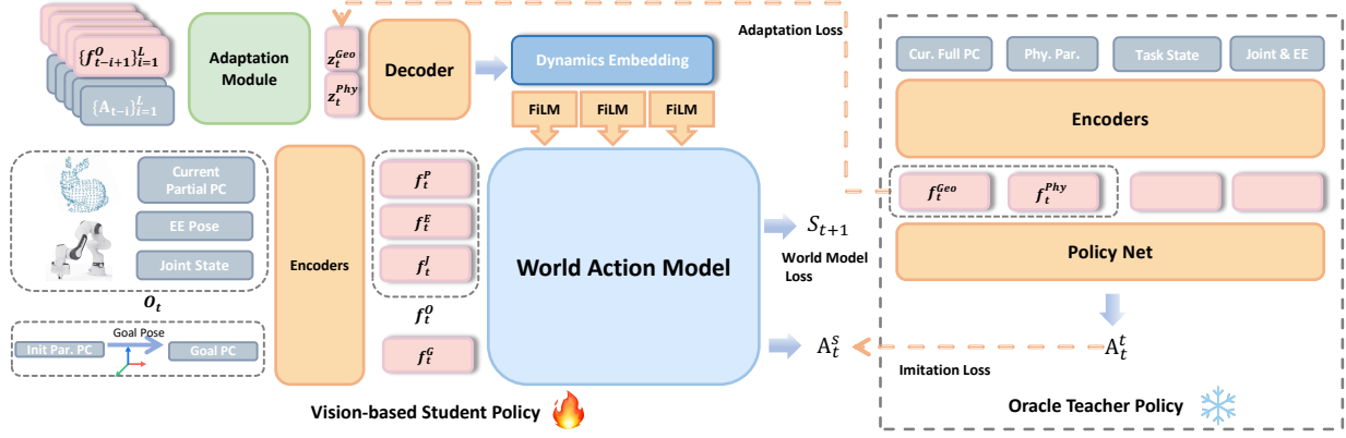
Figure 2. Our World Action Model processes the embeddings of the current observation (partial point cloud, end-effector pose, and joint state) and the goal point cloud (transformed from the initial partial observation) to predict the robot action and next state. Additionally, an adaptation module encodes historical observations and actions, decoding them into the dynamics embedding that conditions the model via FiLM. A pre-trained RL teacher policy (right) supervises both the action and adaptation embedding using privileged full point cloud and physics parameter embeddings.
