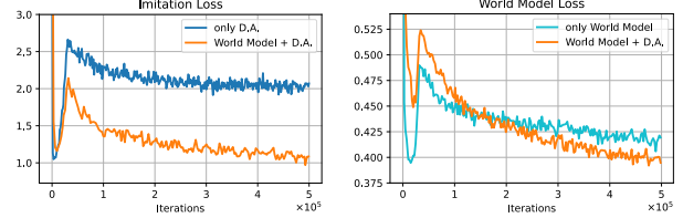
Figure 3. Loss curves during the distillation process. We adopt DAGger which starts with teacher action for execution and gradually adds the weights of student action so that the initial loss declines rapidly. Left: Comparison of imitation loss between using only Dynamics Adaptation and incorporating the World Model. Right: Comparison of World Model loss between using only the World Model and integrating Dynamics Adaptation.
