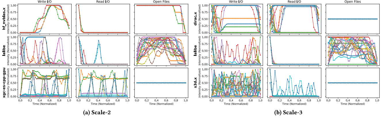
Figure 5: Example of various I/O patterns (write, read, file open) extracted from the ORNL's Darshan traces. Each line in the plot represent an instance of I/O patterns recorded with darshan. Each application shows a set of repeating patterns which we are trying to regenerate by using our proposed generative models.
