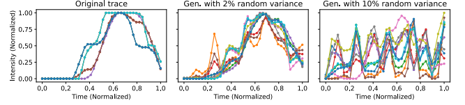
Figure 6: Sensitivity issue with an over-fitted model. We demonstrate how an over-fitted model can generate poor traces due to the small deviations in input. By adding 2% and 10% random noises in the input, the over-fitted model generates very different traces.
