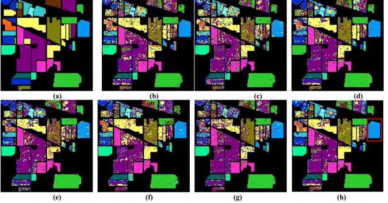
Fig. 8. Visualization of comparative classification results on IP. (a) Ground truth. (b) ResNet. (c) AlexNet. (d) PRAN. (e) DenseNet. (f) FSSFNet. (g) SAGP. (h) TDS-BiGRU.
