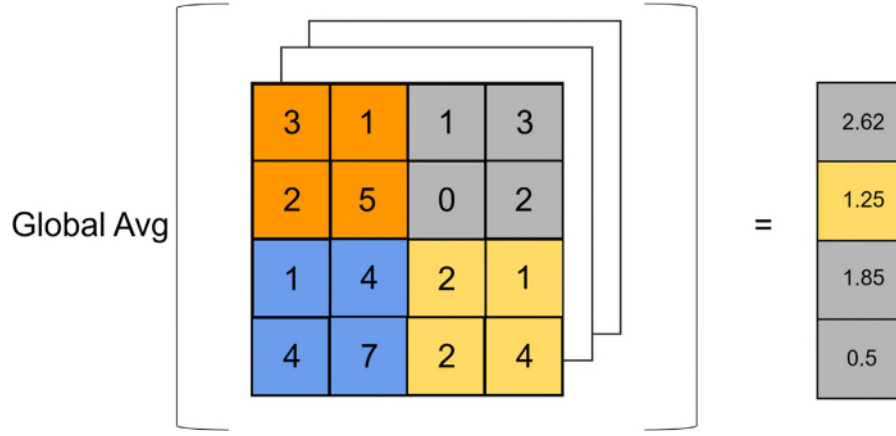
Fig. 4. Global average pooling.
