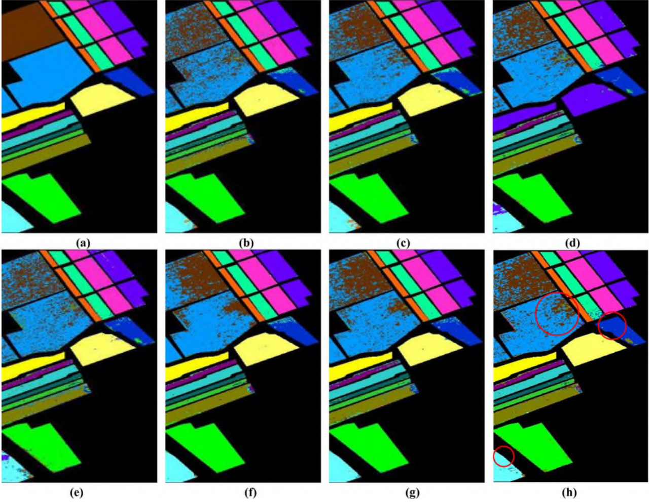
Fig. 10. Visualization of comparative classification results on SA. (a) Ground truth. (b) ResNet. (c) AlexNet. (d) PRAN. (e) DenseNet. (f) FSSNet. (g) SAGP. (h) TDS-BiGRU.
