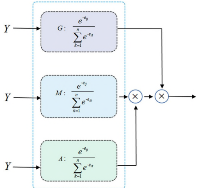
Fig. 3. Three-dimensional Softmax Mechanism module.
