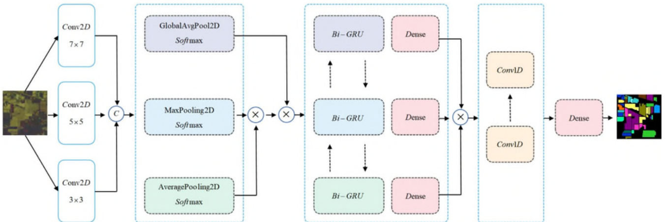
Fig. 1. Schematic of the detailed design of our proposed TDS-BiGRU. represents the multiplication operation. represents the concatenation operation.
