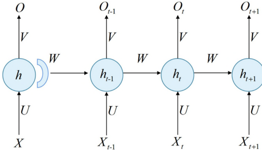
Fig. 5. Schematic diagram of the recurrent unit structure.
