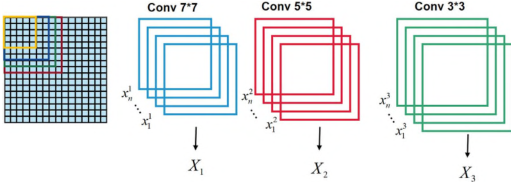
Fig. 2. Schematic diagram of the structure of multi-scale convolution.
