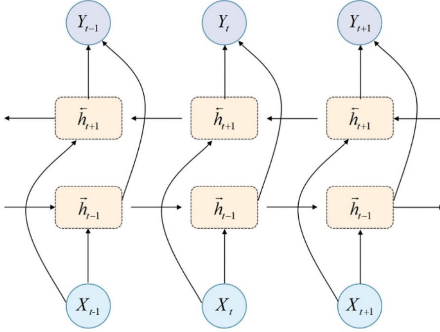
Fig. 6. A schematic diagram of BiGRU, which can be regarded as two unidirectional GRUs, so the hidden layer state of BiGRU at time t is obtained by the weighted sum of the forward hidden layer state and the backward hidden layer state.
