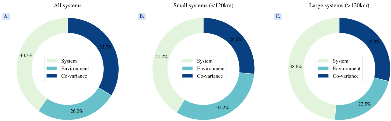
Figure 5. Fraction of the total variance of the DCS maximal extension prediction explained by the system or environmental conditions for (A) all systems, (B) systems smaller than 120 km and (C) larger than 120 km.
