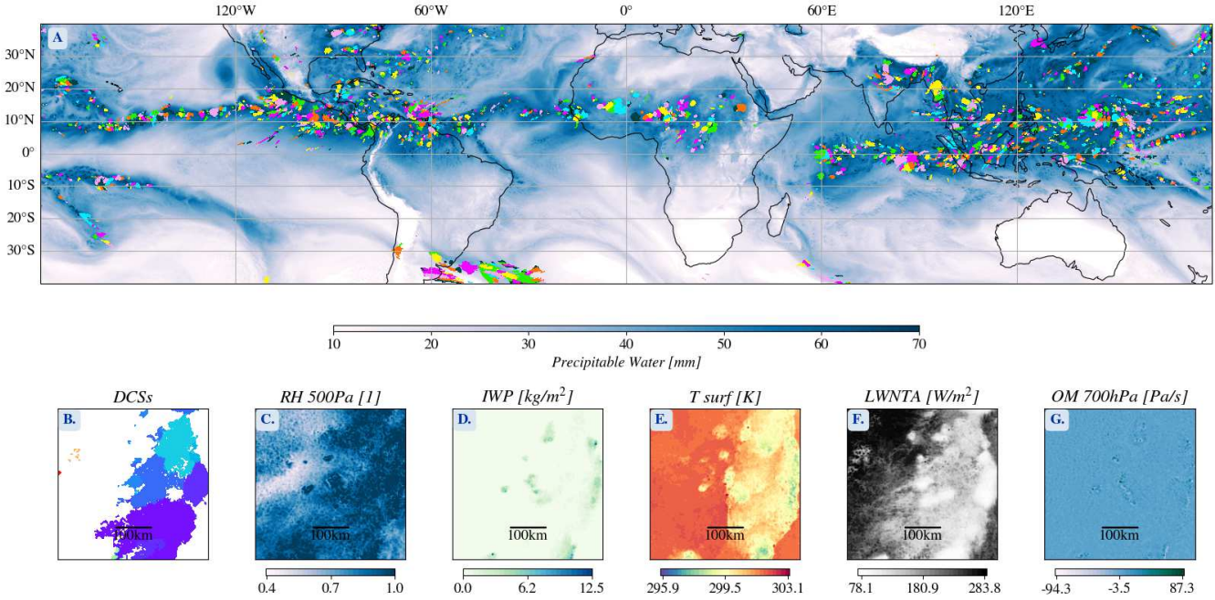
Figure 1. (A) Snapshot from the DYAMOND-SAM summer simulation during August 23 2016 at 23h30 of the Precipitable Water with on top the Deep Convective Systems tracked by TOOCAN focusing only on the tropics. bottom. Example of considered physical fields for a given DCS at 1h of development : (B) the system and its neighbors. (C) relative humidity field. (D) ice water path. (E) surface temperature. (F) long wave emission. (G) vertical velocity at 700 hPa (note the saturated colorbar to ease visualization).
