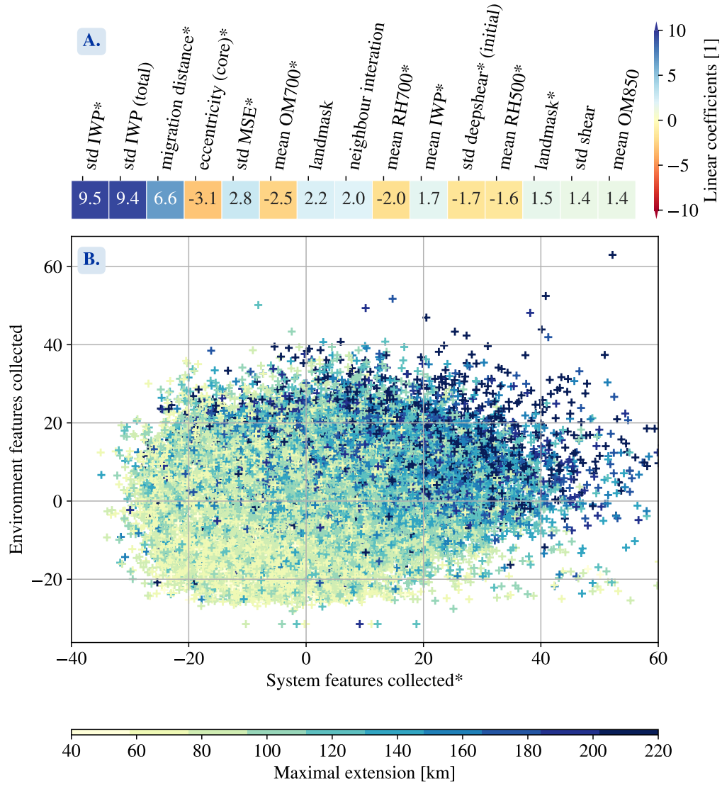
Figure 4. (A) Coefficients optimized for the multi-linear model to solve the supervised task of predicting the maximal extension based on the first 1.5h evolution of DCS growth rate and development features. The coefficients (denoted c_i in [4]) are sorted with their absolute value. There are 15 features displayed, other features are considered negligible (coefficient are below 0.1). These coefficients are applied to normalized input (denoted f_i in [4]). Features with stars are associated with the system's own characteristic, and those without stars are associated with the environment. (B) This figure represents the dependence of the final maximal extension of a given DCS with respect to the initial components from its own characteristics ( x -axis, example : eccentricity, migration distance) and the ones from its initial environment ( y -axis, example : neighbor temperature, mean vertical velocity). It shows that the multi-linear regression is sensitive to both the environment and the system to predict the maximal extension, with a dominant effect from the system itself (stronger gradient in the horizontal direction).
