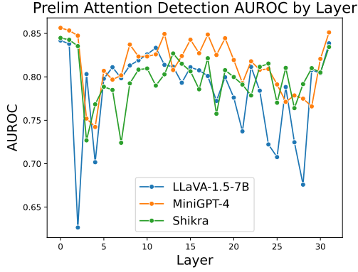
Figure 5. Comparison of different layers’ performance in detecting object hallucination on the MSCOCO dataset.
