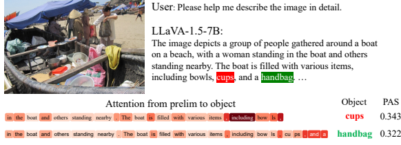
Figure 2. Visualization of Prelim Attention Score (PAS) for a single sample. We show the per-token attention for a suffix of the prelim for a hallucinated and a real object token. Darker red indicates higher attention to the corresponding object token, and a higher PAS score indicates a higher chance of hallucination.
