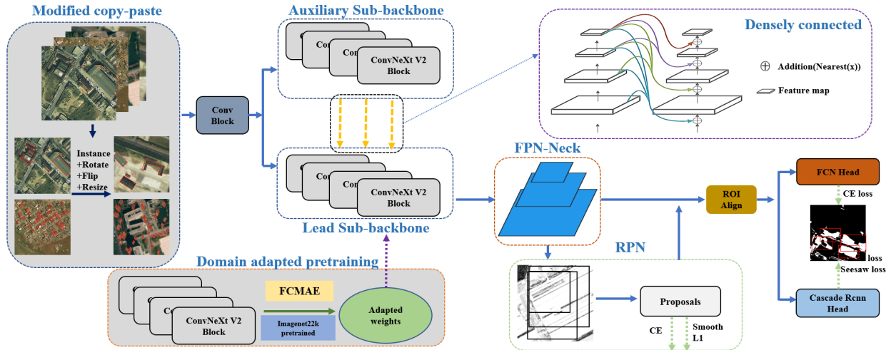
Fig. 4: The overview training workflow and network structure of the Track 1 winning approach.
