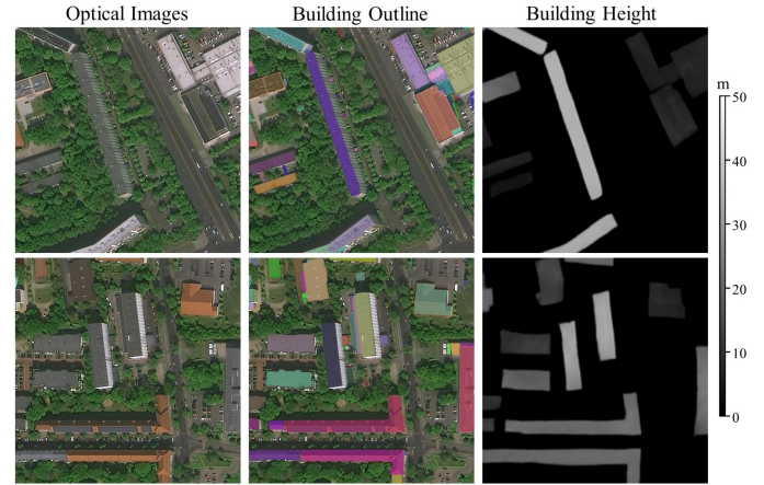
Fig. 12: Qualitative results of the first place of Track 2.
