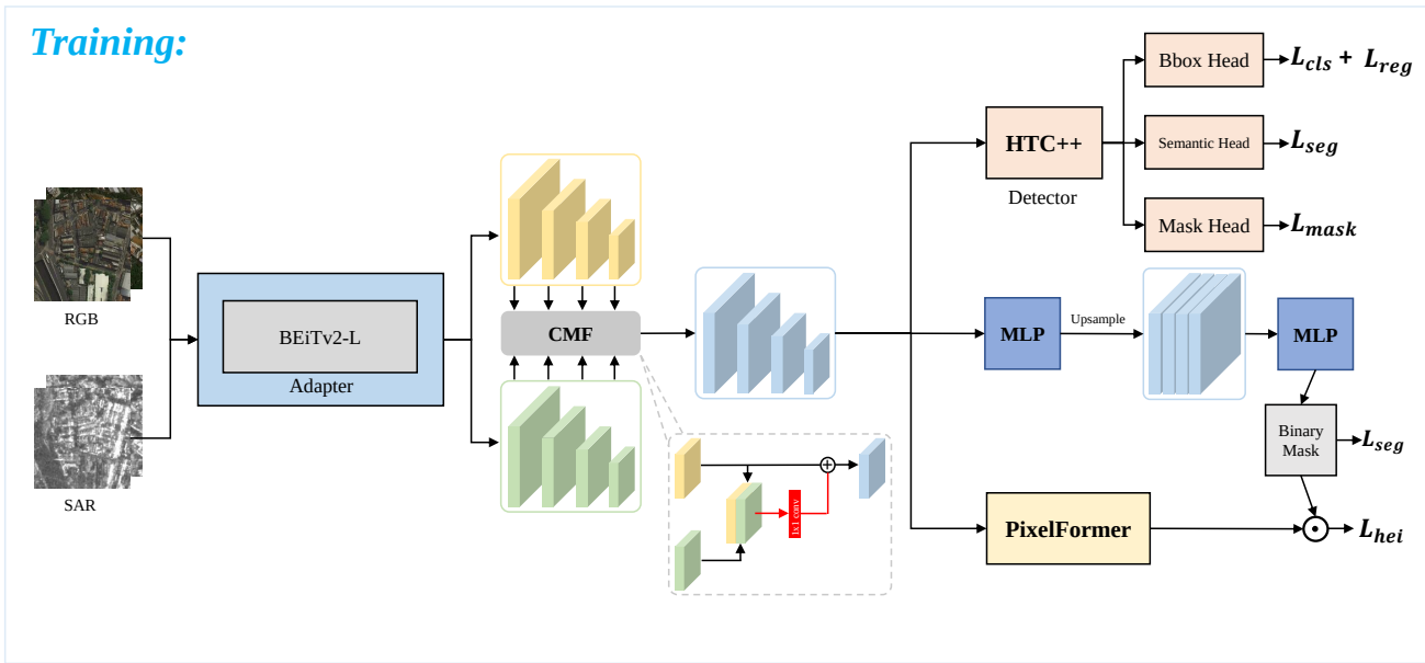
Fig. 13: Illustration of the proposed trident cooperation network (TCNet). The backbone is pre-trained on the DFC23 Track-1 data for initialization. A cross-modal fusion (CMF) module provides more informative shared features for downstream visual tasks. Finally, the trident task-specific heads are leveraged, consisting of a detector [26], a lightweight all-MLP decoder [36], and a pixel query regression head [37]. The binary mask predicted by the all-MLP is additionally used to alleviate foreground confusion existing in the estimated map.
