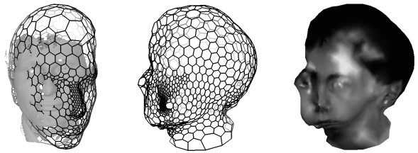
Figure 9. Local deformations
