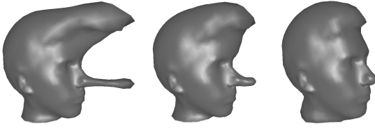
Figure 6. Shape constraint
