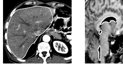
Figure 8. Recovered shapes
