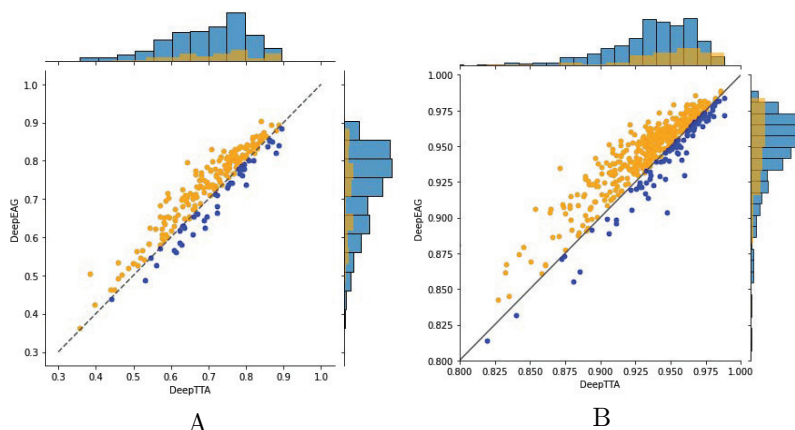
Fig. 4 Pearson’s correlation results for DeepEAG and DeepTTA in independence tests. Each scatter represents a drug or cellline, and its horizontal and vertical coordinates represent Pearson’s correlation results for DeepTTA and DeepEAG, respectively. The scatter at the top left is the case where DeepEAG is better than DeepTTA.
