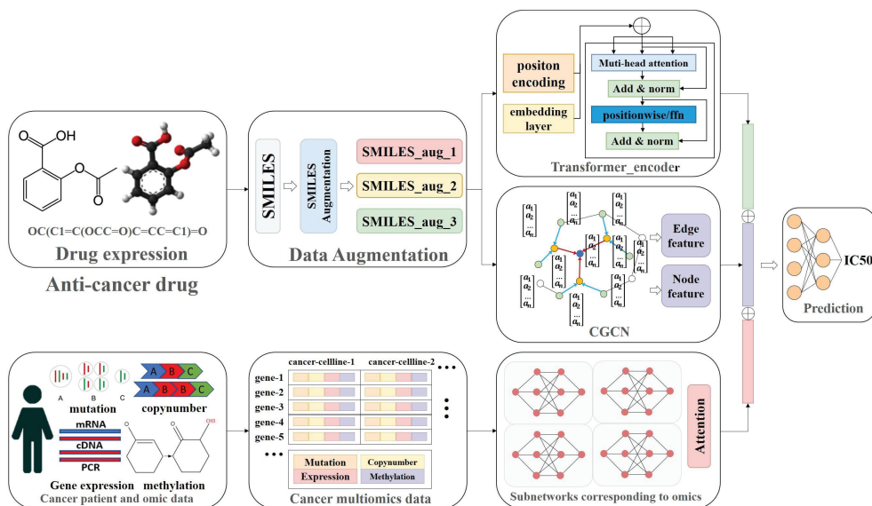
Fig. 1 The framework of DeepEAG. DeepEAG mainly includes three parts: data enhancement, drug feature mining and gene expression feature extraction. The drug feature mining module is divided into CGCN module and transformer module. SMILES expression of cancer drugs is data-enhanced after input and converted into advanced latent characterization by the Encoder and Transformer sections of the GCNC, respectively. The features of cancer cell profiles extracted by the sub-networks are connected and input into the classifier network.
