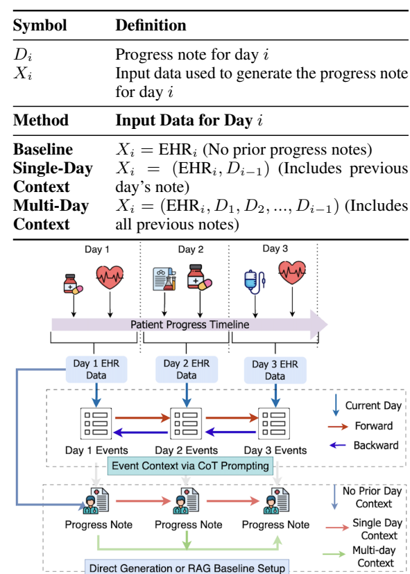
Figure 2: Illustration of the A&P generation workflow (top) and a comparison of input data formulations (bottom).
