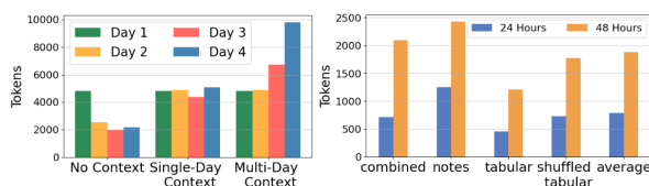
Figure 3: The token length of input data used for A&P generation across days and methods (left), as well as that of input data used for Discharge Summarization across time windows and modalities(right).
