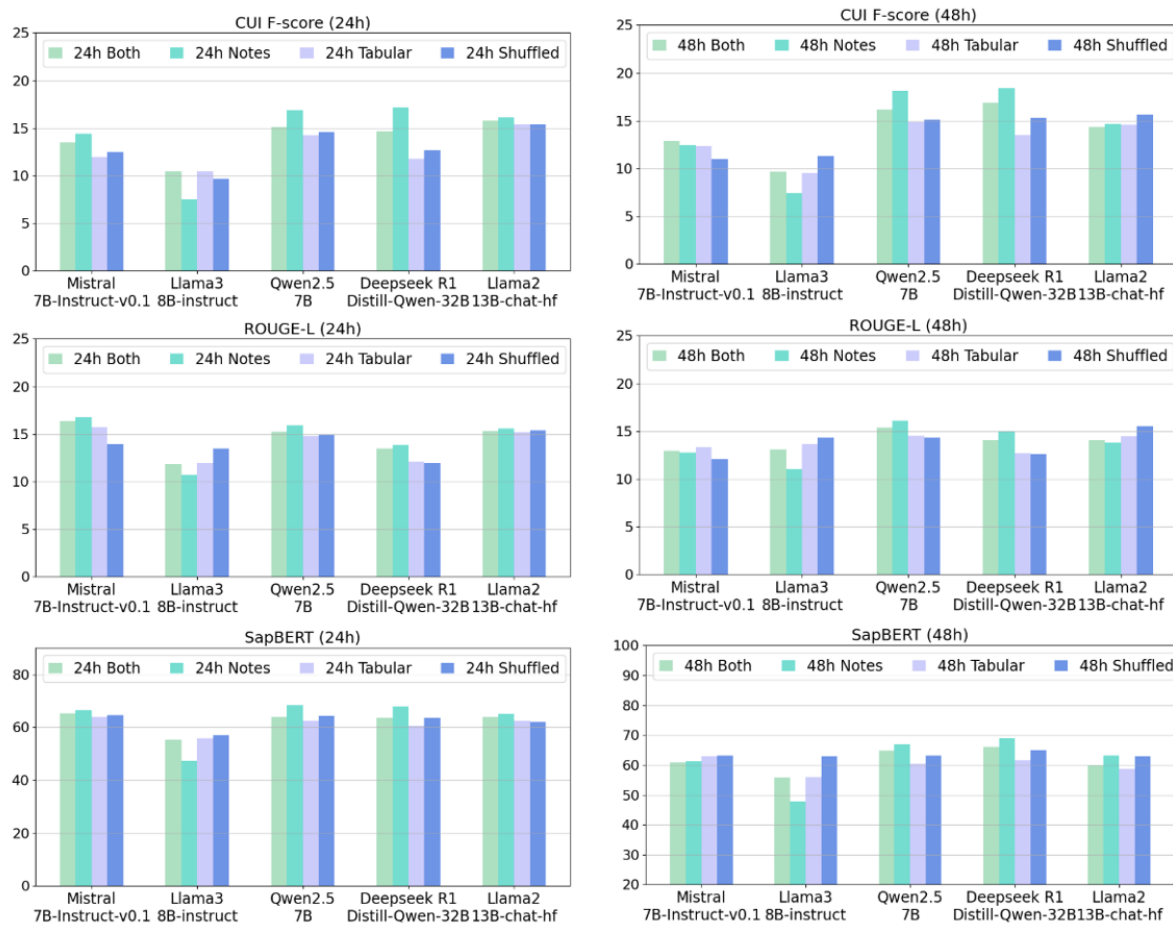
Figure 12: Metric breakdown across modalities for the 24 hour time window (on direct generation)
