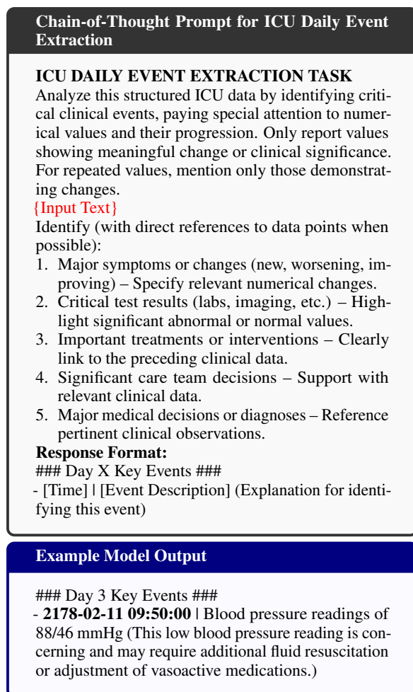
Figure 4: Chain-of-Thought prompting template and example output used for ICU daily event extraction from structured EHR data for A&P generation.
