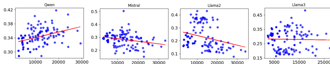
Figure 6: Correlation of token length and average performance across all tasks and metrics
