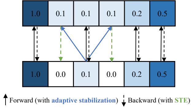
Figure 3: Mechanism of adaptive stabilization and STE. Forward (bottom-up): The adaptive stabilization handles numerical instability by dynamically replacing zero elements in the denominator with the smallest positive value in the sample, preserving maximal dynamic range. Backward (top-down): The STE allows gradients to bypass the replacement operation, treating it as an identity function.
