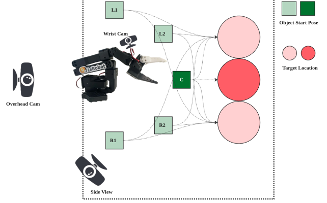
(b) Schematic
