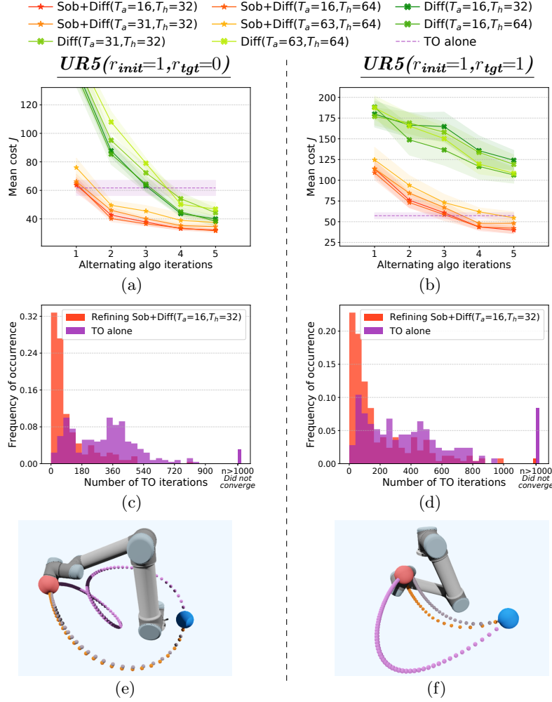
Fig. 3: Interplay algorithm on the UR5. Sob+Diff and Diff are evaluated on the challenging UR5 ( r_{init}=1, r_{tgt}=0 ) (left column), and UR5 ( r_{init}=1, r_{tgt}=1 ) (right column). Methods are tested with varying prediction horizons, T_h = 32 and T_h = 64 , and action lengths T_a : 16, 31, and 63 (as T_a \leq T_h - T_o and T_o = 1 ). For UR5 ( r_{init}=1, r_{tgt}=0 ), n_{traj} = 50 in the first three iterations and 100 after, for UR5 ( r_{init}=1, r_{tgt}=1 ) n_{traj} is doubled, in both cases n_{pl} = 10^4 . Sob+Diff solves both tasks, even with a large number of applied actions ( T_a = 63 ) for fast inference. (c) and (d) report the number of TO iterations taken to converge, with Sob+Diff and without , showing that Sob+Diff helps the solver quickly converge. (e) and (f) show an instance of each task, in blue the initial position, in red the goal, in pink trajectories obtained by TO alone (representing trajectories used at the beginning of training), in orange Sob+Diff trajectories, in gray refined ones. Sob+Diff trajectories are more direct, avoiding local minima.
