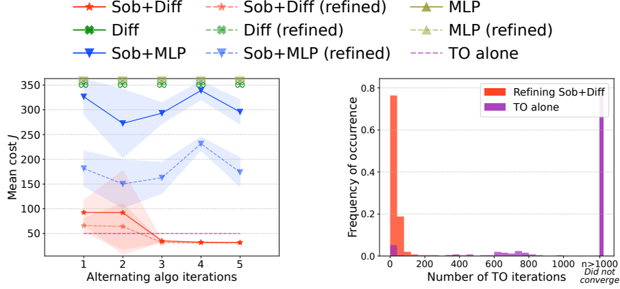
(a) Mean cost w.r.t. algo iters, evaluating both the policy and refined , i.e. TO starting from the policy solution.
