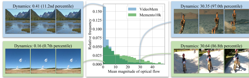
Fig.3. Video distribution by level of motion for VideoMem and Memento10k. The motion metric for each video is calculated by averaging optical flow magnitude over the entire video. A high percentage of videos in the VideoMem dataset are almost static, while Memento10k is much more balanced. We show select examples with low and high levels of motion.
