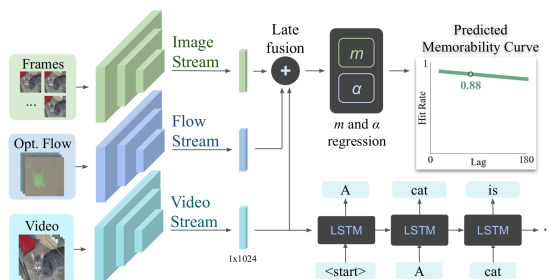
Fig. 8. The architecture of SemanticMemNet. An I3D is jointly trained to predict memorability and semantic captions for an input video. Its memorability predictions are combined with a frames-based and optical flow stream to produce m_{80} and \alpha , the parameters of the memorability decay curve.
