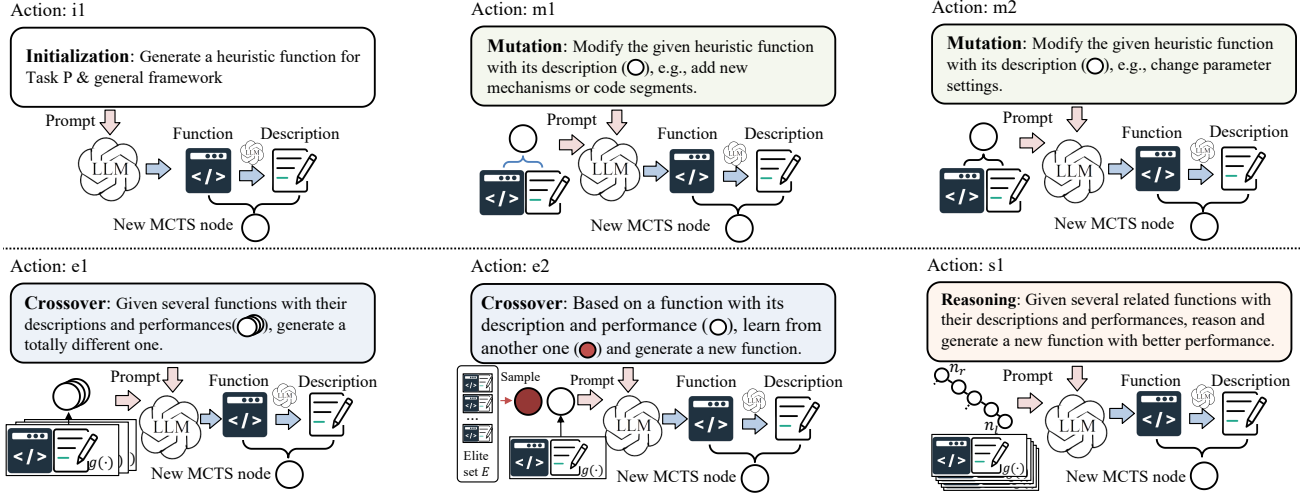
Figure 2. LLM-based actions in MCTS-AHD for heuristic evolution. Actions include initializing a new heuristic (i1); two mutation actions (m1 and m2) to mutate an existing heuristic function into a new one with diverse mechanism or detail settings; two crossover actions (e1 and e2) to generate a new heuristic from multiple existing ones; and a novel tree-path reasoning action (s1) to get a better heuristic function from organized function samples on an MCTS tree path from the root node n_r to a leaf node n_l .
