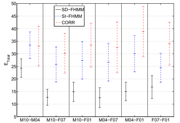
Figure 1: Total error for each speaker pair of 600 test speech mixtures using correlogram-based multipitch tracking (CORR) and speaker dependent and independent FHMM-based multipitch tracking (SD-FHMM and SI-FHMM, respectively).
