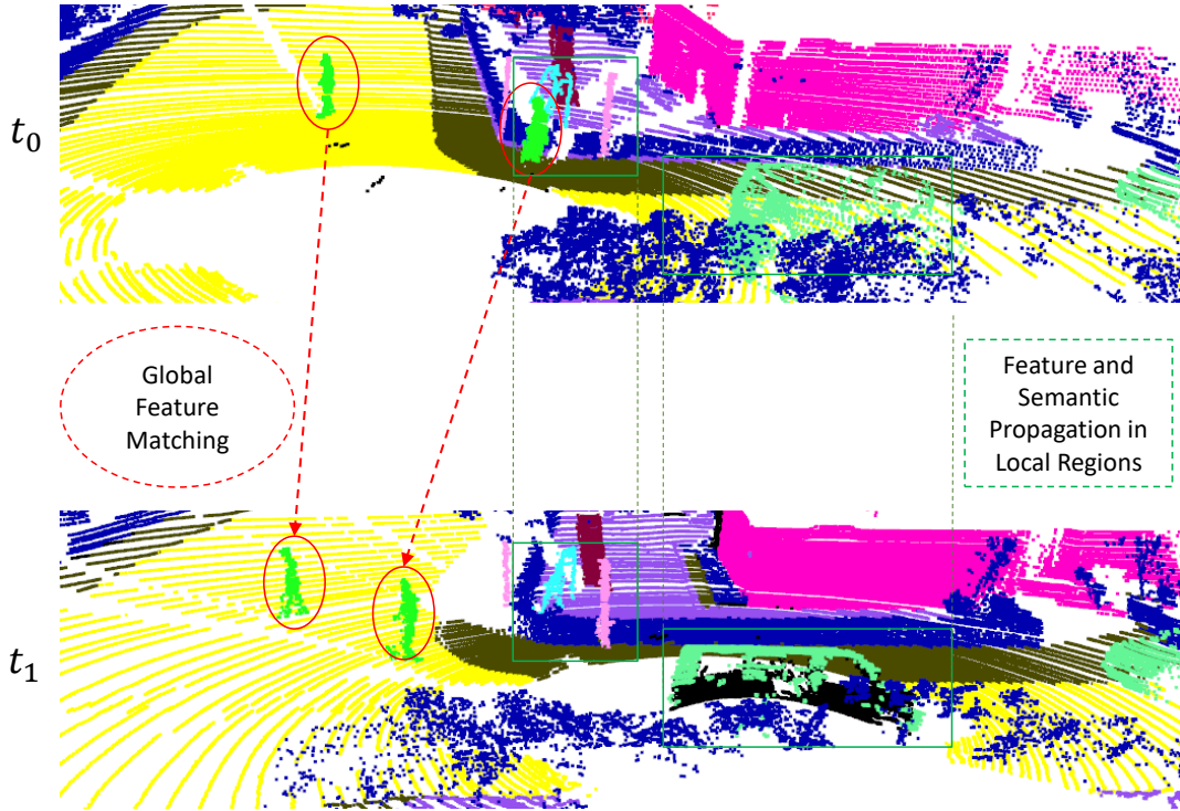
Fig. 2. An illustration of the temporal information captured in our method. As indicated by the red circles, the global temporal matching module builds the connections between the moving people in different locations and times. As indicated by the green rectangles, the feature and semantic propagation module propagates the information of the local regions in the previous frame to the current frame.
