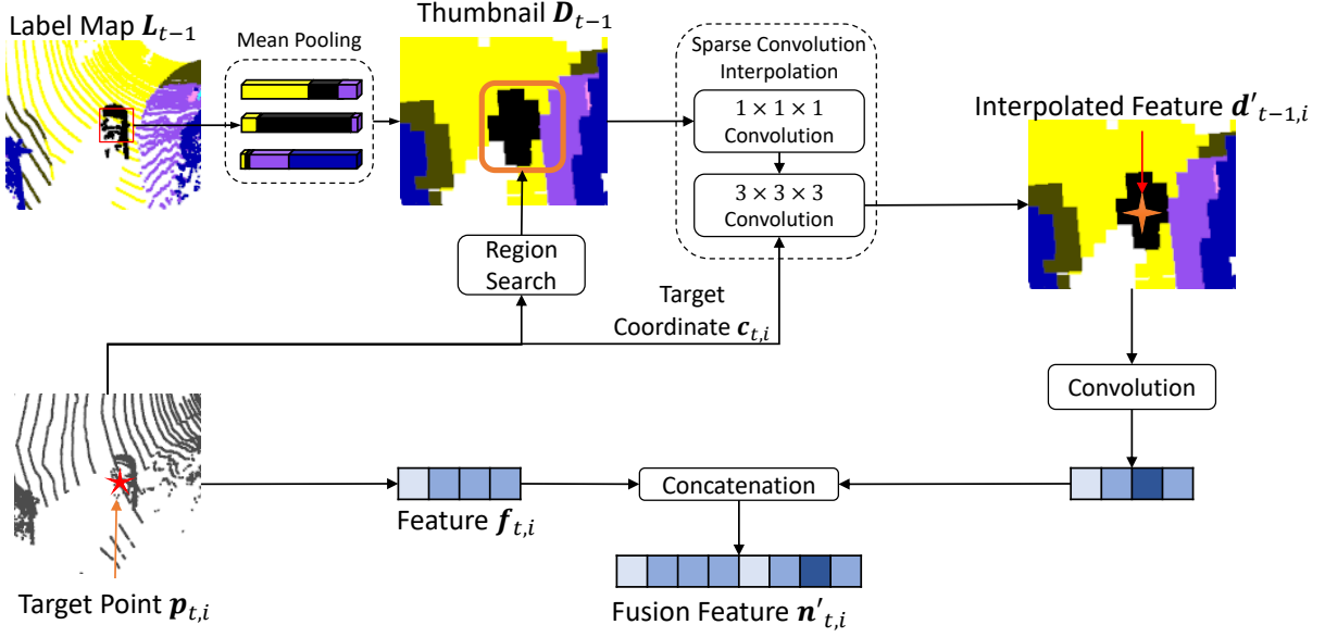
Fig. 6. An explanation for local semantic propagation. Similar to Figure 4, the red star is the target point and the area in the orange region is the interpolation area. Distribution map D_{t-1} is a statistics for L_{t-1} .
