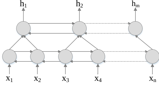
Figure 2: The structure of the encoder.
