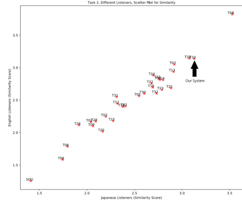
Figure 4: Scatter plot matching similarity of Japanese listeners and English listeners for task 2 of VCC 2020.
