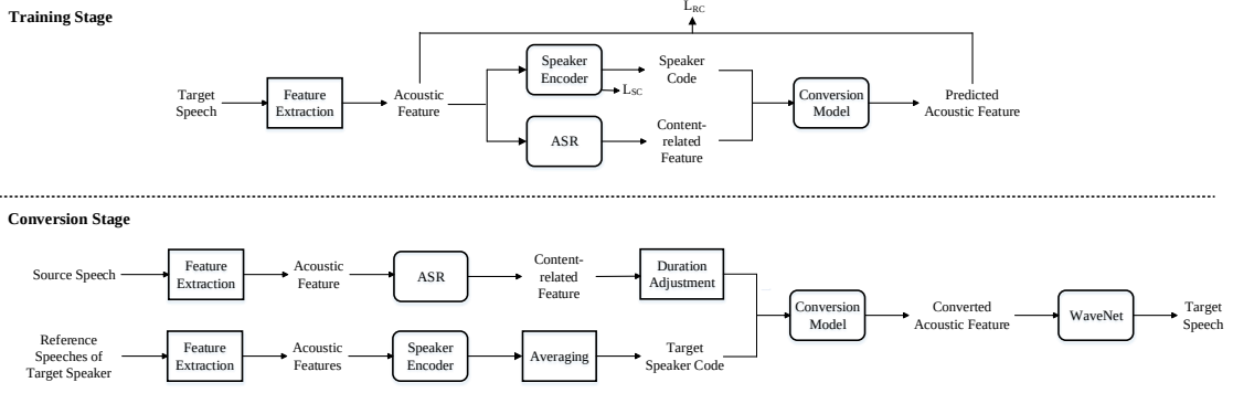
Figure 1: The framework of the proposed system.
