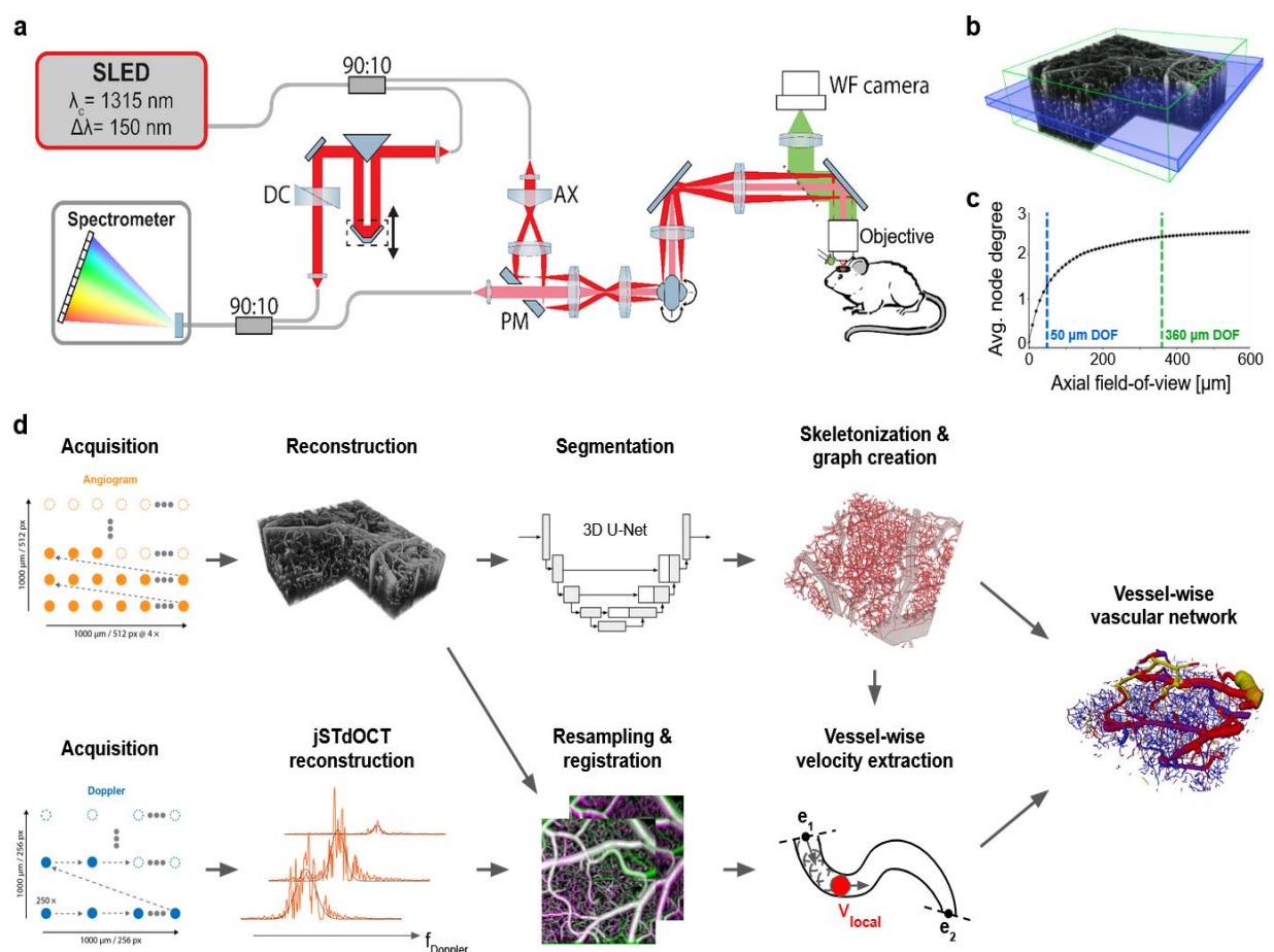
Figure 1: Overview of the xf-irOCM and processing pipeline. a) Schematic of the xf-irOCM. In the sample arm, illumination and detection light paths are decoupled using a pierced mirror (PM) and depicted in dark and light red, respectively. AX: axicon, DC: dispersion compensation b) OCTA volume acquired with the xf-irOCM. The green box emphasizes the in-focus volume achieved with our xf-irOCM, resulting in a depth-of-field of \approx 360 \mu\text{m} . The blue box represents the simulated in-focus volume ( \approx 50 \mu\text{m} ) of a standard OCM system with equivalent lateral resolution. The lateral dimensions are 1000 \mu\text{m} \times 1000 \mu\text{m} . c) Average node degree of the vascular networks from Blinder et al. 1 over increasing axial field-of-view. These vascular networks serve as a reference to estimate the necessary axial FOV to duly capture vascular network characteristics. The dashed green and blue lines highlight the extended depth-of-field and regular depth-of-field shown in (b), respectively. d) Acquisition and automatic processing pipeline that enables extraction of vessel morphology and functional flow information in each vessel, combining OCTA and DOCT.
