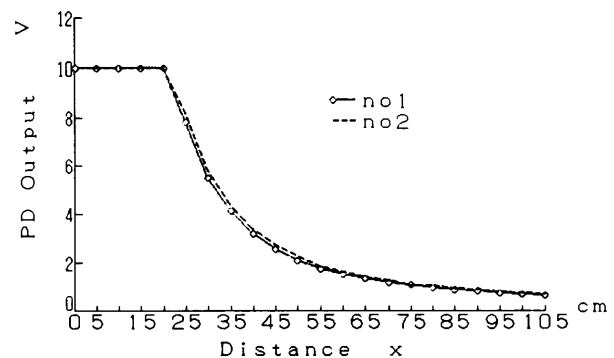
Fig. 13 Output of photodiode dependent on LED distance
