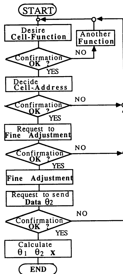
Fig. 8 Algorithm for communication in undocked state
