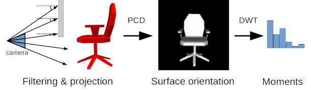
Figure 3. Baseline method for single observation model
