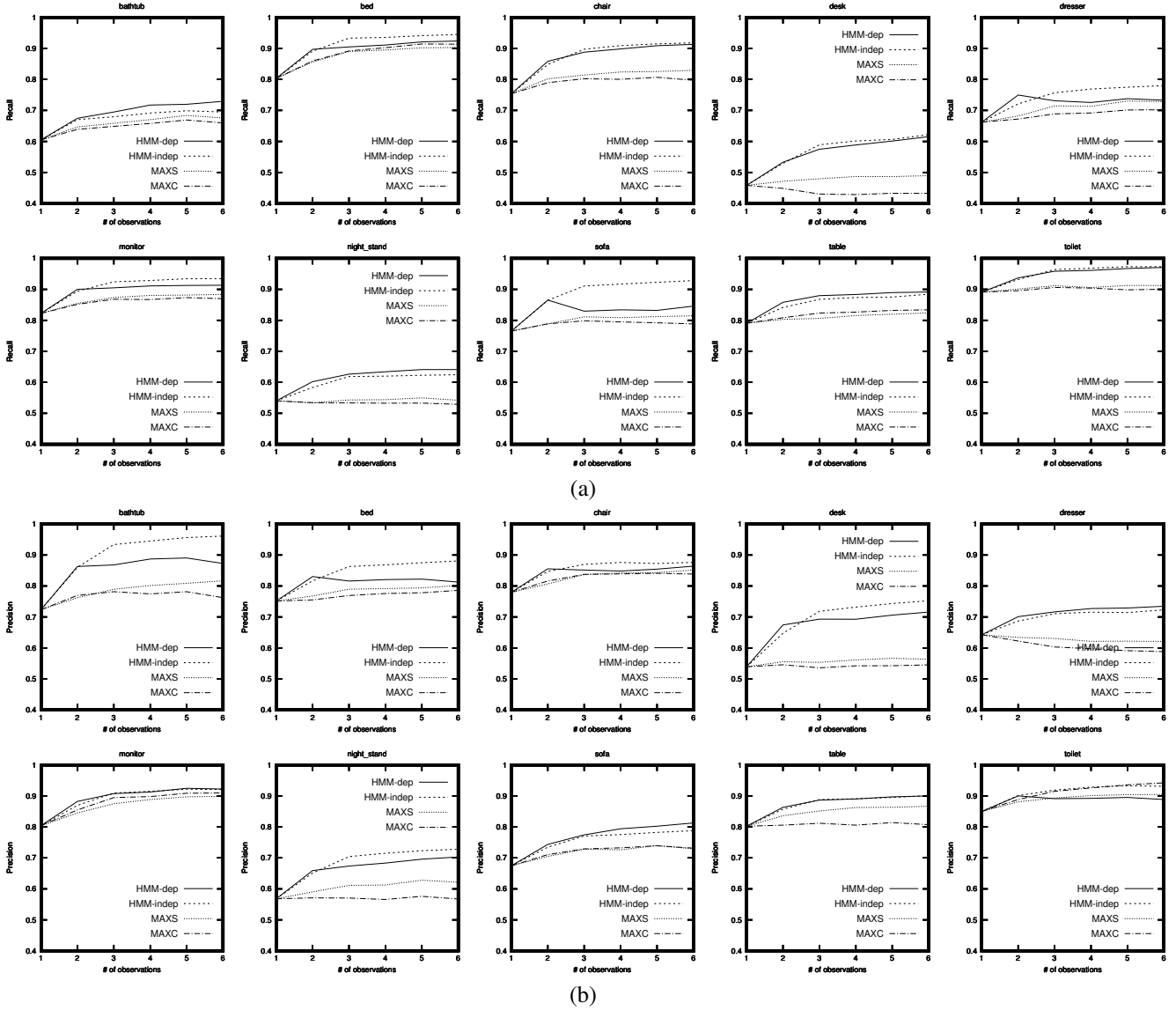
Figure 4. Comparison of multi-view hypothesis fusion schemes; (a) Recall and (b) Precision
