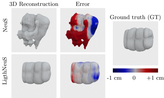
Fig. 2. Benefits of illumination decline. Result on the “ Cecum 1 a ” sequence. Top: The NeuS reconstruction exhibits multiple artifacts that make it unusable. Bottom: Our reconstruction is much closer to the ground truth shape. The error is shown in blue if the reconstruction is inside the surface, and in red otherwise. A fully saturated red or blue denotes an error of more than 1cm and grey denotes no error at all.
