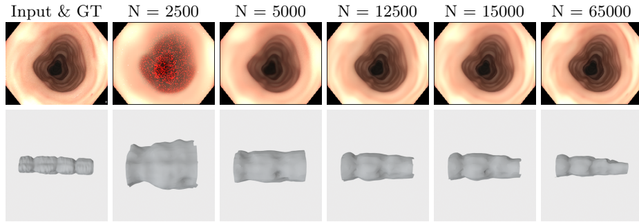
Fig. 5. Reconstruction convergence. Results on “ Transcending 1 a ” sequence. We show the intermediate results for N optimisation iterations. We see how the reconstruction converges quickly. In 65k iterations we already have a reasonable solution, compared to the 300k iterations proposed by the authors of NeuS.
