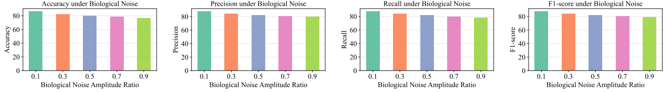
Figure 7. Variations in Accuracy, Precision, Recall, and F1-score on the DeepShip dataset under biological noise. Each color represents a different biological noise amplitude ratio under the same experimental configuration.
