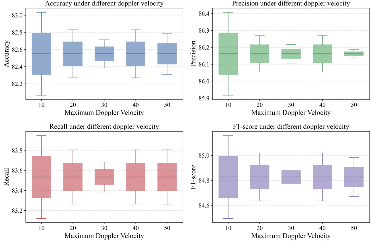
Figure 8. Variations in Accuracy, Precision, Recall, and F1-score on the DeepShip dataset under Doppler-induced spectral distortion. Each boxplot visualizes the distribution of performance metrics obtained under different maximum target velocities ( v_{\max} = 10\text{--}50 ), where Doppler shifting is simulated by time-scaling the waveform to emulate frequency compression or expansion caused by source-receiver relative motion. The boxes indicate the interquartile range (IQR), the central line denotes the median, and whiskers represent non-outlier ranges. Across all Doppler velocities, the metrics exhibit minimal spread and consistent central tendencies, demonstrating that the proposed model is highly robust to spectral deformation induced by Doppler effects.
