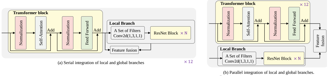
Figure 4. Illustration of local-global branch integration strategies: (a) serial integration, where the local and global branches are fused sequentially; and (b) parallel integration, where both branches operate concurrently before fusion.
