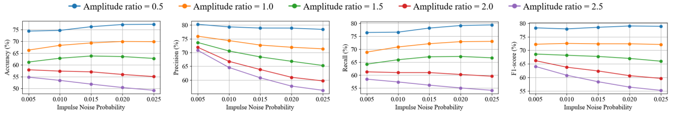
Figure 6. Performance variations of Accuracy, Precision, Recall, and F1-score on the DeepShip dataset under impulse noise. The x-axis indicates the impulse noise probability, while each colored line represents a different impulse noise amplitude.
