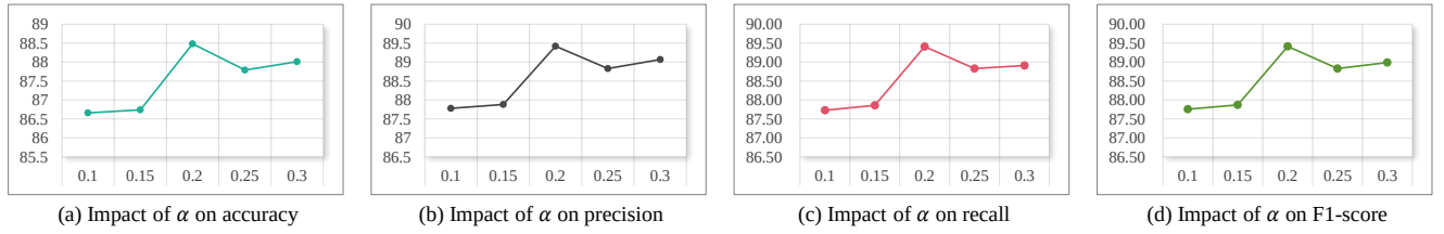
Figure 3. Performance variation with respect to the fusion hyperparameter \alpha across accuracy, precision, recall, and F1-score.
