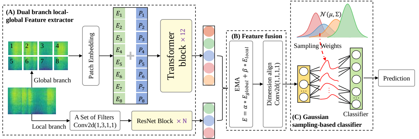
Figure 2. Overview of the proposed framework for underwater acoustic target recognition. The architecture comprises (A) a dual-branch local–global feature extractor, (B) a feature fusion and alignment module, and (C) a Gaussian sampling-based classifier.
