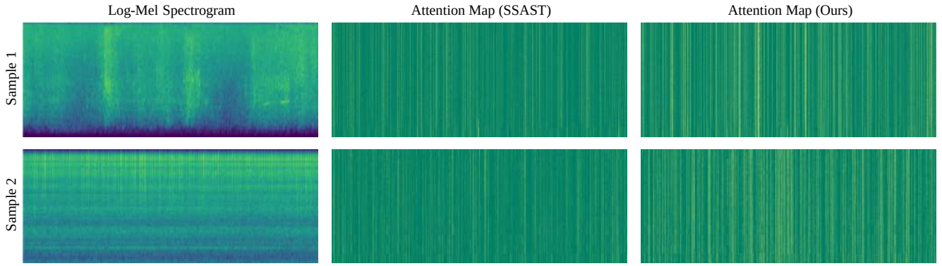
Figure 1. Visualization of class activation maps on the log-Mel spectrogram, highlighting important time–frequency regions in comparison between the baseline SSAST and our hybrid local-global representation learning framework.
