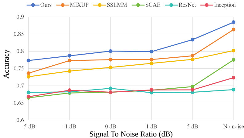
Figure 5. Accuracy vs. SNR on Deepship dataset under additive white noise.
