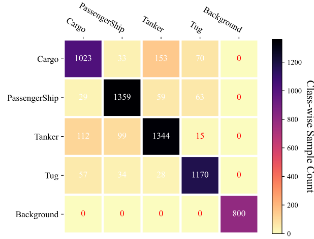
Figure 9. Confusion matrix for proposed model on deepship dataset.
