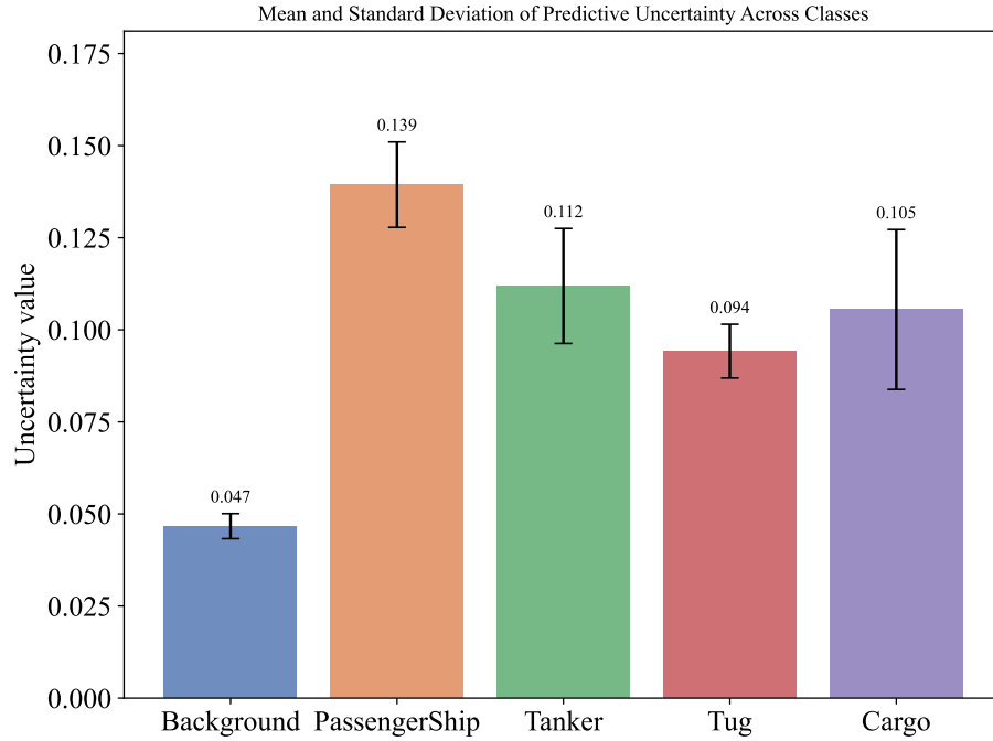
Figure 11. Uncertainty analysis using five stochastic forward passes. Samples with low predictive variance correspond to confident and correct decisions, while high-variance predictions align with misclassifications or ambiguous cases, offering a reliable cue for uncertainty-aware decision-making.
