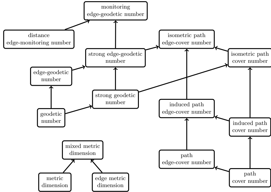
Fig. 1. Relations between the parameters discussed in the paper. If a parameter A has a directed path to parameter B , then for any graph, the value of A is upper-bounded by a linear function of the value of B .
