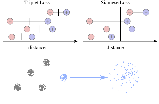
Figure 3: At the top, the conceptual threshold is shown in the case of both a triplet (left) and a Siamese (right) loss. At the bottom, the localized-context problem is illustrated in a two-dimensional descriptor space. The blue cluster is expanded (increasing d_p ) and pushed away from the other clusters (increasing d_n ). Therefore, the performance \rho_{\text{sub}} = d_n - d_p increases slightly even though the scaling of the descriptors has deteriorated.
