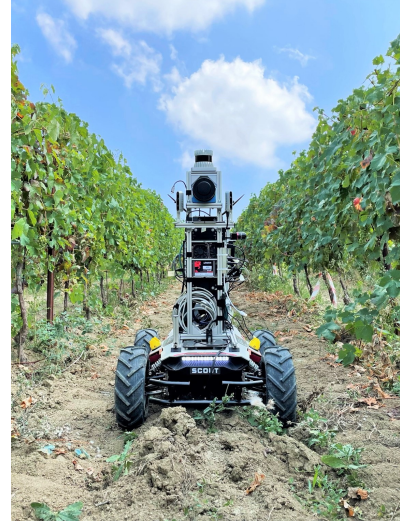
Fig. 1. Our robotic platform navigating a real vineyard.
