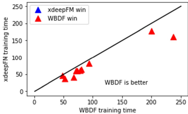
Fig. 5 Training time comparison between WBDF and xdeepFM
