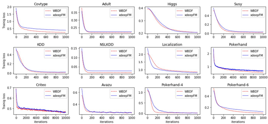
Fig. 4 Comparison of the training-loss convergence profile of WBDF and xdeepFM
