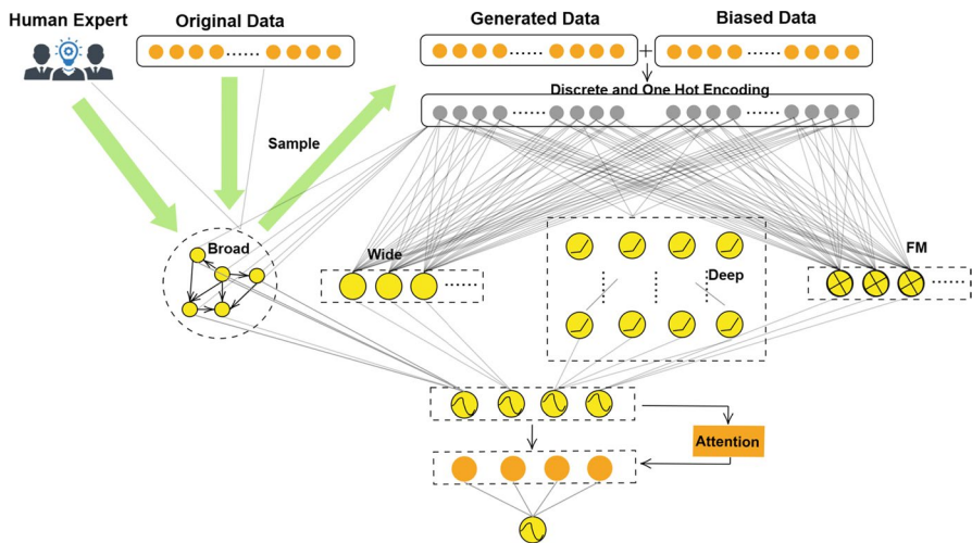
Fig. 3 Illustration of knowledge-guided application of WBDF
