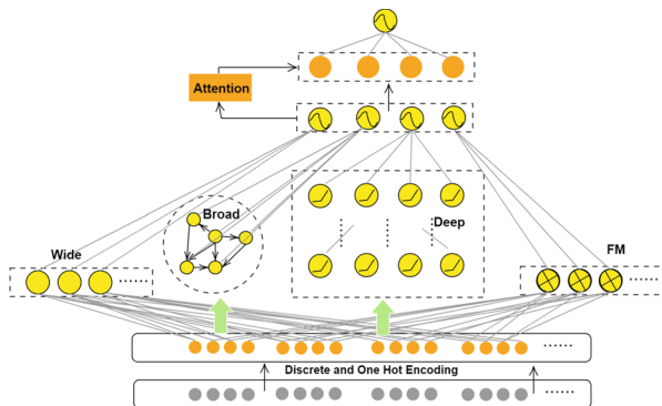
Fig. 1 Illustration of the WBDF framework
