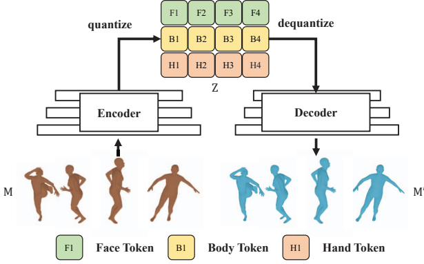
Figure 3. The pre-processing stage of M-Adaptor. The motion tokenizer contains a VAE-based encoder E and a decoder D for quantization and dequantization. Each token Z_i of time i can be split as body motion token B_i , facial expressions token F_i , and hand gesture token H_i
