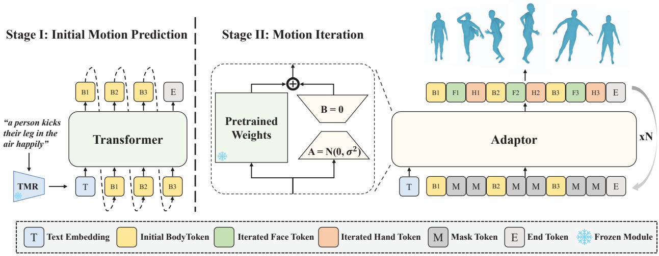
Figure 2. The architecture of our generator M-Adaptor. It first generates sequences of coarse-grained body motion tokens from pre-trained text embedding in stage I, then iterates the mask tokens to yield more accurate sequences of fine-grained motion tokens, including body motion, facial expressions, and hand gestures in stage II.
