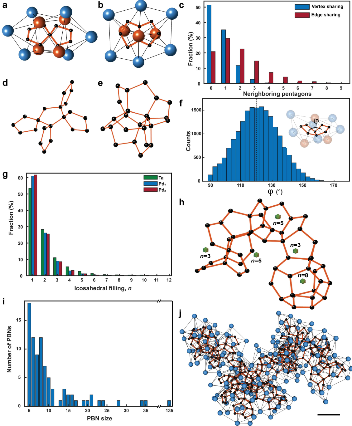
Fig. 5 | Direct observation of pentagonal bipyramid networks in monatomic amorphous materials. a, b , Vertex- and edge-sharing of the five-fold skeletons, which share four and five atoms with their neighbours, respectively. The capping atoms are in
