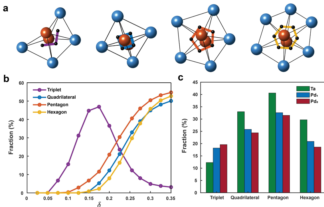
Fig. 2 | Polytetrahedral packing in the amorphous Ta film and two Pd nanoparticles.
