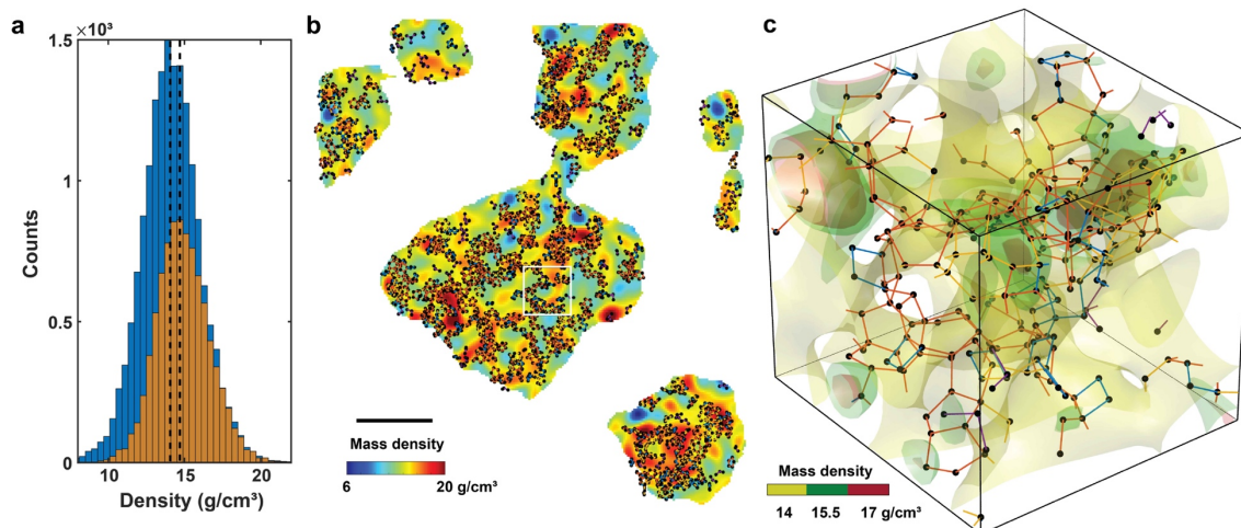
Fig. 3 | Correlation of 3D local mass density heterogeneity and polytetrahedral packing. a , Mass density distribution in the regions of the amorphous Ta film with (yellow) and without polytetrahedral packing (blue), where polytetrahedral packing increases the average mass density by 3% (dashed lines). b , A slice through the Ta film shows the local mass density heterogeneity (colour) overlaid with polytetrahedral packing (black). c , 3D surface rendering of local mass density heterogeneity magnified from the square region in (b) , which is overlaid with three- (purple), four- (blue), five- (orange) and six-fold (yellow) skeletons. Scale bar, 2 nm.
