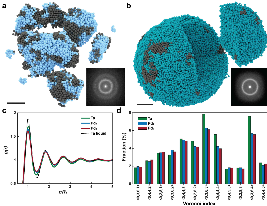
Fig. 1 | Determination of the 3D atomic structure of monatomic amorphous materials. Experimental 3D atomic model of an amorphous Ta film (a) and a Pd nanoparticle (Pd 1 ) (b) with surface crystal nuclei in grey. The two insets show the average 2D power spectra of the experimental images for the Ta film and Pd 1 nanoparticle, where the amorphous halo is visible. Scale bars, 2 nm. c, PDFs of the Ta film (green), two Pd nanoparticles (Pd 1 in blue and Pd 2 in red) and an MD simulated Ta liquid at 5200 K (dotted curve). The PDFs were normalized by the Ta and Pd atom size. d, 12 most populated Voronoi polyhedra in the three samples, where the Voronoi index is arranged with the increase of the coordination number. All the analysis in (C), (D) and Figs. 2-6 are based on the amorphous regions of the three samples with the crystal nuclei removed.
