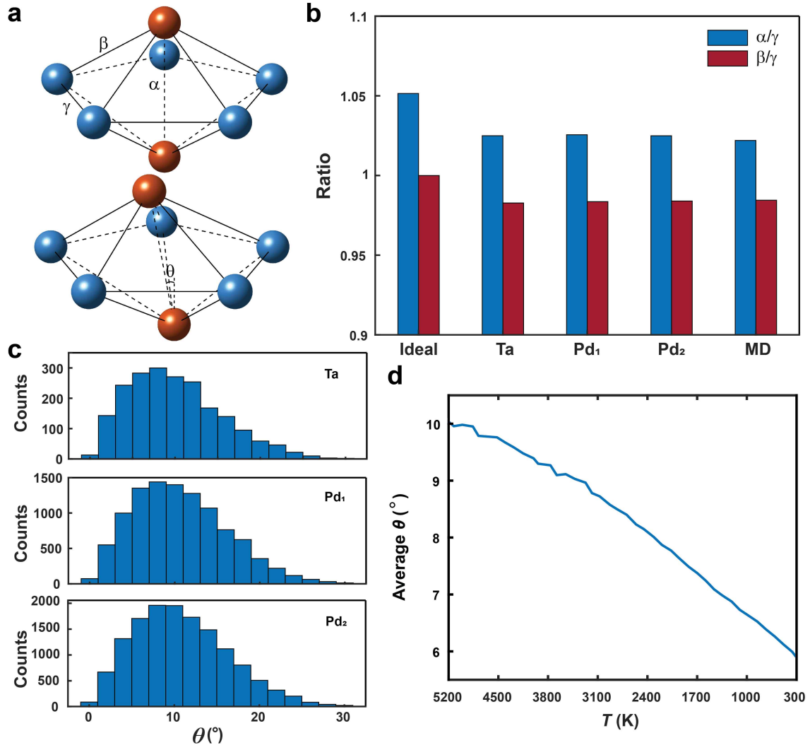
Fig. 4 | Quantitative characterization of 3D atomic packing of pentagonal bipyramids. a , An ideal pentagonal bipyramid (top) consisting of two capping (brown) and five ring atoms (blue). \alpha , \beta and \gamma represent the capping, capping-ring and ring atom bonds, respectively. Bottom shows the average pentagonal bipyramid of the amorphous Ta film, where the \alpha bond and the plane of five ring atoms form an angle ( \theta ). b , The \alpha/\gamma and \beta/\gamma ratios of an ideal pentagonal bipyramid as well as those in the amorphous Ta film, Pd 1 , Pd 2 nanoparticles and the MD simulated Ta liquid at 5200 K. c , Distribution of \theta in the Ta film (top), Pd 1 (middle) and Pd 2 (bottom) nanoparticles with the average \theta of 10.0°,
