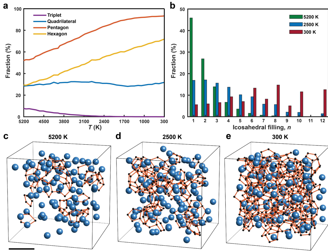
Fig. 6 | Pentagonal bipyramids networks in the MD simulated Ta liquid and metallic glass. a , Population of the four most abundant atomic motifs (triplets, quadrilateral, pentagonal and hexagonal bipyramids) as a function of the temperature. b , Population of pentagonal bipyramids filling partial icosahedral sites ( n ) at the liquid temperature (5200 K), during quench (2500 K) and at room temperature (300 K). c-e , Snapshot of a fraction of the 3D atomic models and PBNs at the above three temperatures. Ta atoms are shown as blue balls and the PBNs as orange lines and black dots. The PBNs quickly grow in size and form more icosahedra with the decrease of the temperature. Scale bar, 4 Å.
