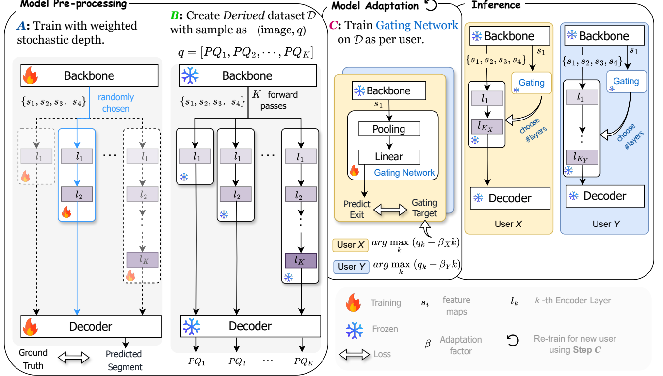
Figure 3. ECO-M2F framework. During the model pre-processing phase, we train the model to exit stochastically at K potential exits using Step A. Next, in Step B, we use this model to perform inference on the training images at each exit to create a dataset \mathcal{D} . In the model adaptation phase, we perform Step C to establish a gating target based on the computational budget and train a lightweight gating network. During inference , the network exists at the layer designated by the gating network.
