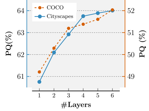
Figure 4. Intuition for Eq. (4). This figure shows that prioritizing PQ requires more encoder layers, while fewer layers lead to poorer PQ. (Backbone: SWIN-T; training set).
