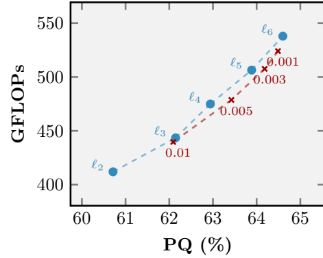
Figure 5. ECO-M2F outperforms M2F with WSD by effectively reducing computation without compromising performance, as shown by the varying results with the Gating module across different \beta values. (Dataset: Cityscapes)
