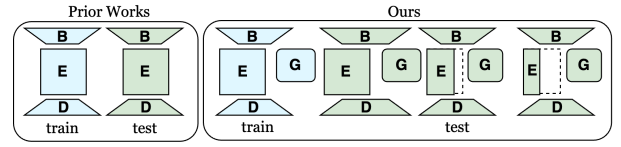
Figure 1. Comparison to prior works. Instead of conventional M2F-style architecture that provides a “one-size-fits-all” solution, our method ECO-M2F trains models to run directly at various resource encoder depths by leveraging a gating function. B , E , D , and G denote the backbone, encoder, decoder, and (our proposed) gating network, respectively.
