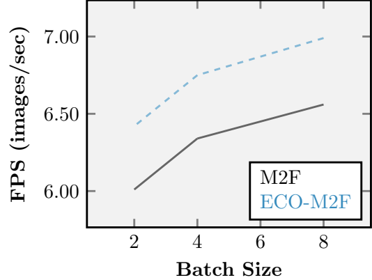
Figure 6. FPS vs. batch size. ECO-M2F consistently achieves higher FPS than M2F [6] across all batch sizes. (Dataset: Cityscapes; Backbone: Res50)
