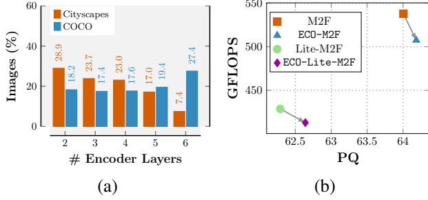
Figure 2. (a) Histogram of images achieving best panoptic segmentation by the number of encoder layers. (b) Our method demonstrates superior performance and lower computational cost compared to the baseline models. (Dataset: Cityscapes; Backbone: SWIN-T)
