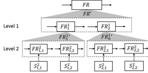
Figure 4. A two-level example system to describe the hierarchical functional requirements decomposition process.
