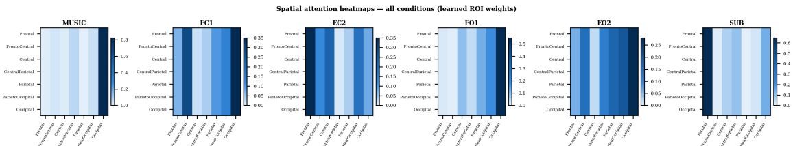
Figure 2. Spatial attention heatmaps (7 \times 7) averaged across all attention heads and test subjects per condition. The highest-weighted ROI consistently matches the most important ROI from the removal analysis.
