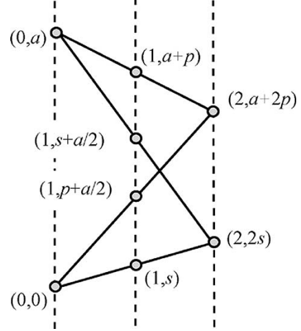
Fig. 13. Quadrilateral in a lattice finite geometry.
