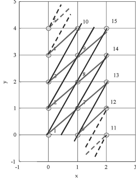
Fig. 2. An example of the rectangular grid for q = 5 and c = 3 .
