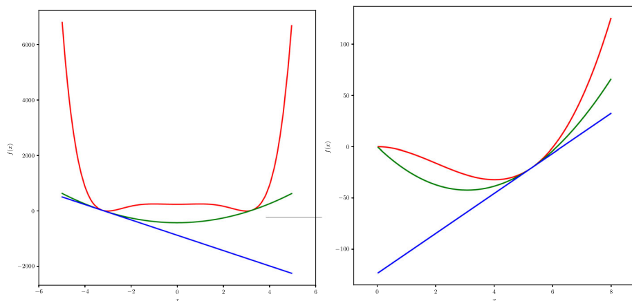
Fig. 5 Quadratic underestimators (green) for the univariate d.c. functions f(x) = (27x^2 + x^6 + 250) - 15x^4 at x_0 = -3.24 (left) and f(x) = x^3 - 6x^2 at x_0 = 5.24 (right), compared to linear underestimators (blue) using the “S” method
