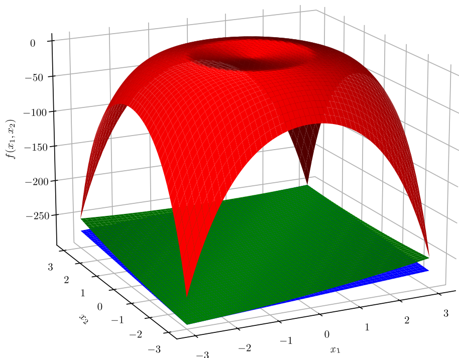
Fig. 7 The pathological d.c. function from problem sisser , where no locally convex point of construction admits a valid quadratic underestimator unless a method with shift is employed. The green surface depicts the quadratic underestimator generated using the shift-utilizing “DS” method at a central point, \mathbf{x}_0 = [0.592, 0.555] , whereas its linear relaxation counterpart (i.e., after dropping the second-order term) is shown in blue
