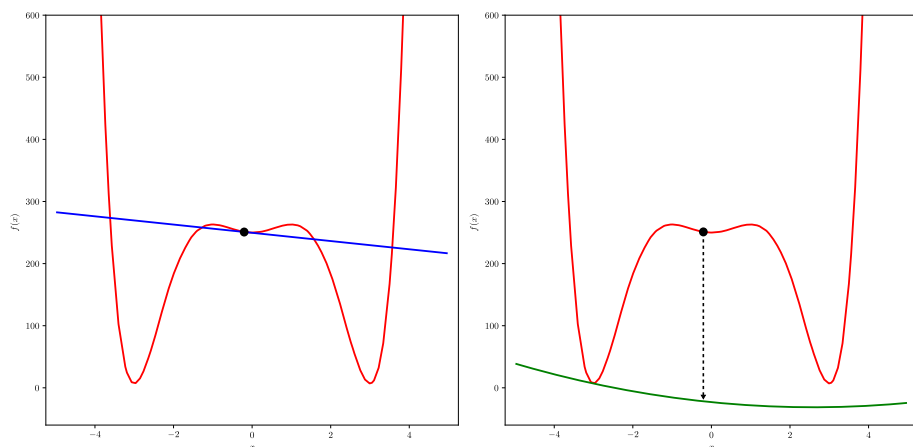
Fig. 2 Introducing the shift parameter allows the construction of a valid quadratic underestimator (right, in green) for the d.c. function f(x) = (27x^2 + x^6 + 250) - 15x^4 at x_0 = -0.125 even when, at the same point of construction, a linear underestimator is not valid (left, in blue)
