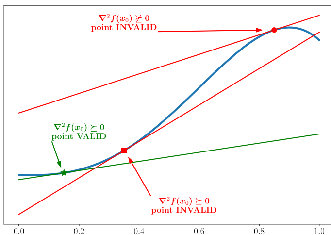
Fig. 1 The univariate non-convex d.c. function f(x) := 3x^3 - 2.5x^4 over the domain x \in [0, 1] with first-order Taylor series approximations constructed at (i) x = 0.15 , (ii) x = 0.35 , and (iii) x = 0.85 , illustrating respectively three different cases: (i) underestimation over the entire domain, (ii) overestimation in part of the domain despite local convexity at the point of construction, and (iii) overestimation where the point of construction is not locally convex
