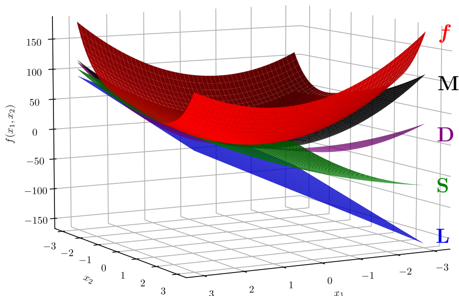
Fig. 4 Qualitative evidence highlighting the improvement in the quality of underestimators by using more general methods from our hierarchy. The d.c. function f(x_1, x_2) = (x_2^4 + 9x_1^2 + 2x_2^2) - 2(x_1 + x_2)^2 is underestimated in the box domain [-3, 3]^2 using (1.84, -1.04) as the point of construction. Here, “ f ” is the function, “ L ” is the linear underestimator, while “ S ”, “ D ”, and “ M ” are the quadratic underestimators constructed using the respective methods
