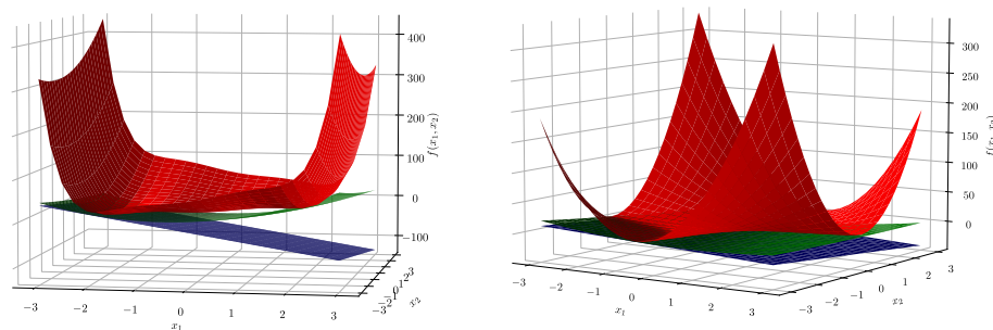
Fig. 6 Quadratic underestimators (green) for the bivariate d.c. functions f(\mathbf{x}) = (15.0x_1^2 + 9x_2^2 + x_1^6) - [3(x_1 + x_2)^2 + 6.3x_1^4] at \mathbf{x}_0 = (-1.95, -1.81) (left) and f(\mathbf{x}) = [5x_1^2 + 5x_2^2 + \frac{3}{2}(x_1^2 + x_2^2)^2] - [4(x_1 + x_2)^2 + \frac{3}{2}x_1^4 + \frac{3}{2}x_2^4] at \mathbf{x}_0 = (-0.68, -2.21) (right), compared to linear underestimators (blue) using the “S” method
