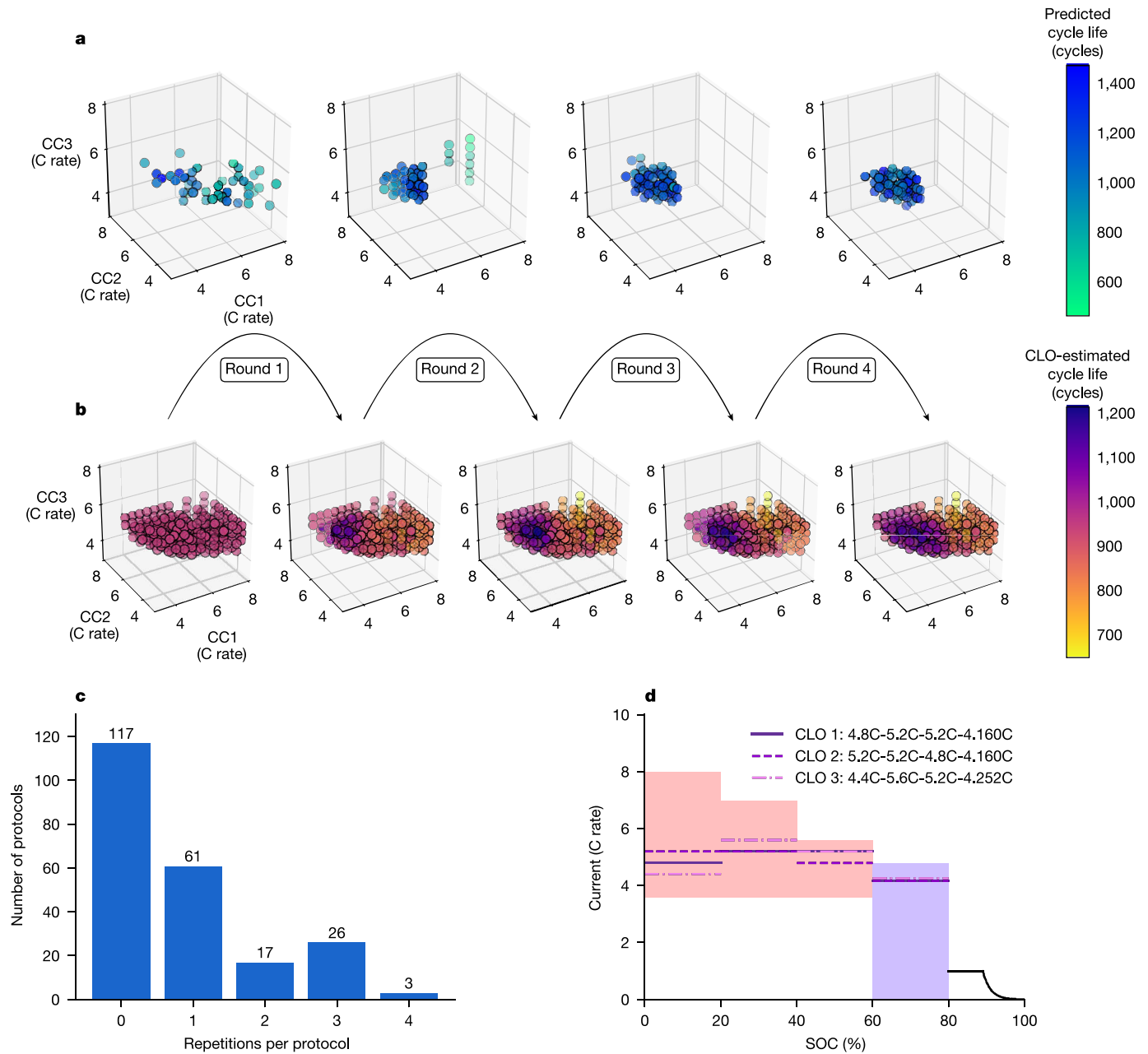
Fig. 3| Results of closed-loop experiments. a, Early cycle life predictions per round. The tested charging protocols and the resulting predictions are plotted for rounds 1–4. Each point represents a charging protocol, defined by CC1, CC2 and CC3 (the x , y and z axes, respectively). The colour scale represents cycle life predictions from the early outcome prediction model. The charging protocols in the first round of testing are randomly selected. As the BO algorithm shifts from exploration to exploitation, the charging protocols selected for testing by the closed loop in subsequent rounds fall primarily into the high-performing region. b, Evolution of the parameter space per round. The colour scale represents cycle life, as estimated by the BO algorithm. The initial cycle life
