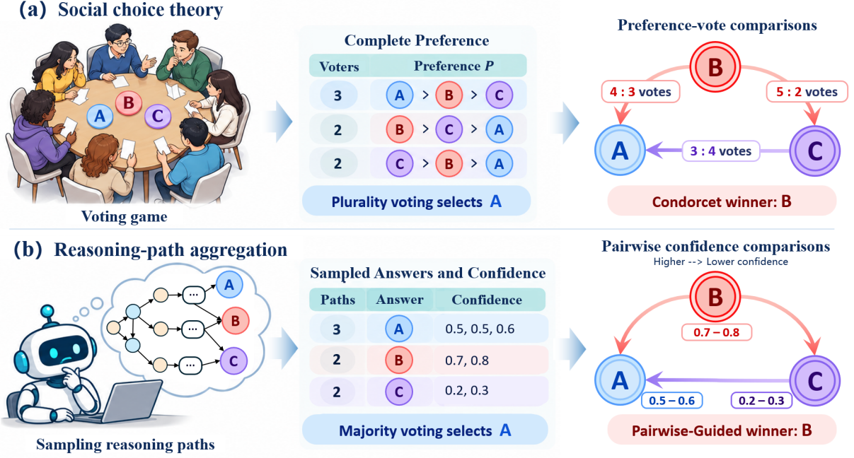
Figure 1: From voting support to pairwise comparative evidence. (a) Plurality voting selects A , whereas pairwise preference comparisons identify B as the Condorcet winner. (b) Sampled reasoning paths provide answers and confidence scores. Pairwise confidence comparisons complement voting support, enabling the proposed aggregation method to select B .
