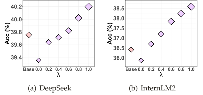
Figure 7: Effect of confidence reliability in pairwise comparisons on accuracy, averaged over three math datasets.
