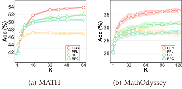
Figure 6: Scaling behavior under varying numbers of sampled reasoning paths K on MATH and MathOdy. using InternLM2-Math-Plus-7B.
