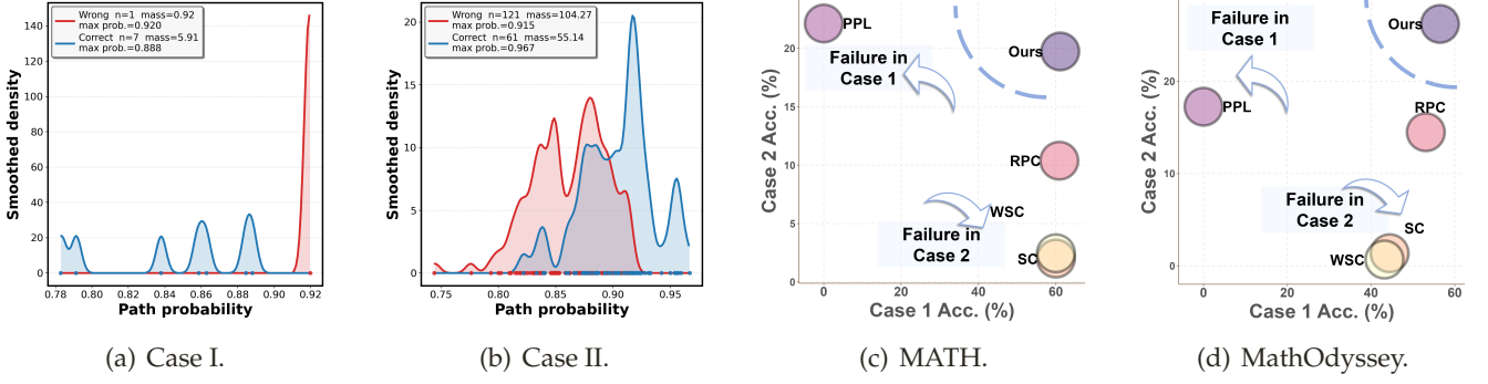
Figure 8: Complementary roles of voting support and pairwise confidence comparisons. In Case I, an incorrect answer contains the highest-confidence path despite weaker voting support. In Case II, an incorrect answer has stronger or tied voting support, while pairwise confidence comparisons favor a correct answer. The last two panels report the corresponding behavior on MATH and MathOdyssey.
