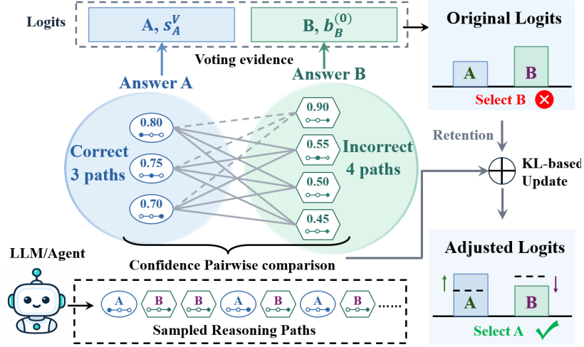
Figure 9: Illustration of PGLA.
