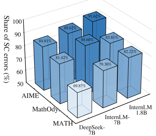
(b) percentage of SC error
