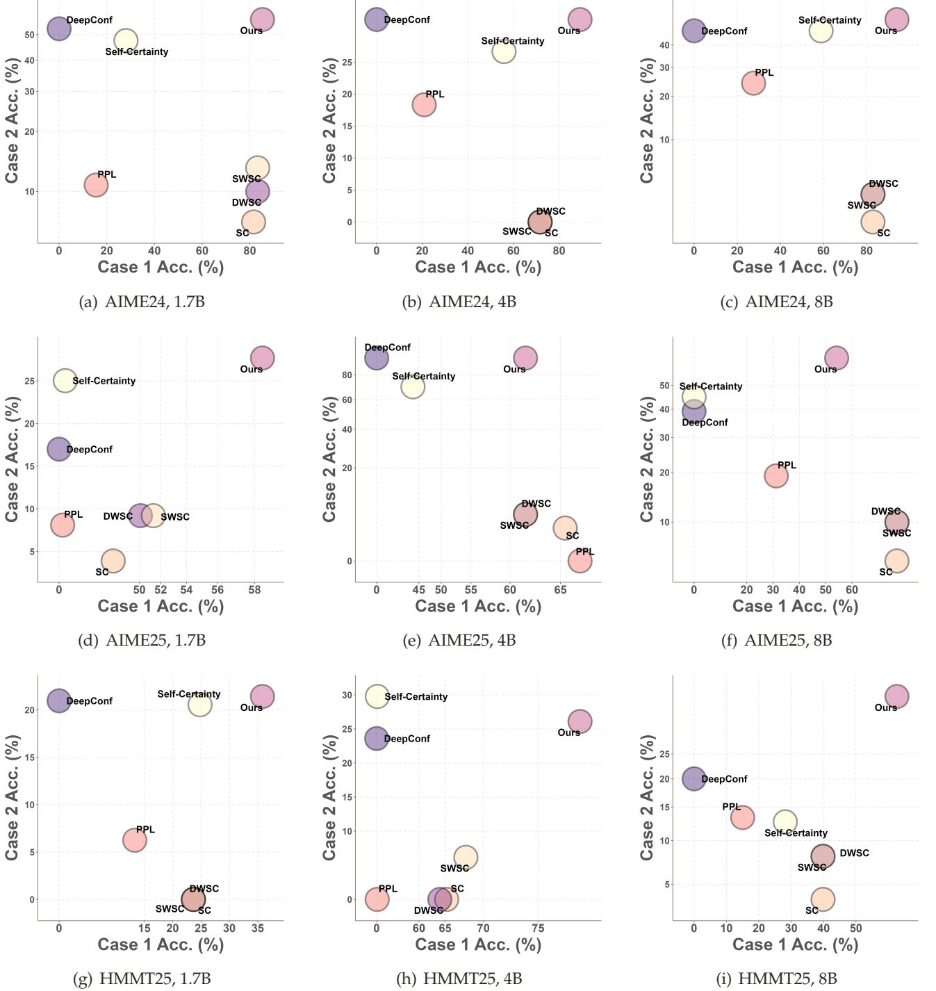
Figure 10: Tradeoff between Case I and Case II on AIME24, AIME25, and HMMT25 using Qwen3-1.7B, Qwen3-4B, and Qwen3-8B. Ours denotes PGLA. DeepConf, PPL, and Self-Certainty denote DeepConf Best-of- N , PPL Best-of- N , and Self-Certainty Best-of- N , respectively. SWSC and DWSC denote Self-Certainty-Weighted SC and DeepConf-Weighted SC, respectively.
