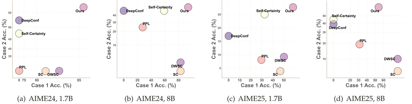
Figure 5: Tradeoff between Case I and Case II on AIME24 and AIME25 using Qwen3-1.7B and Qwen3-8B. DWSC denotes the DeepConf-Weighted SC method.
