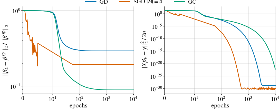
Figure 6. Sparse recovery in noiseless regression with \gamma = 0.1 . Left: normalized recovery error. Right: normalized training loss. GC achieves substantially lower recovery error although it converges slower compared to (S)GD.
