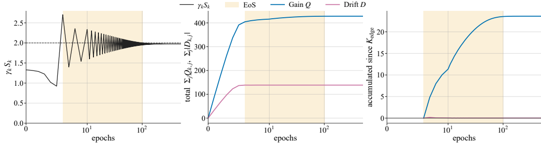
Figure 9. Following the onset of EoS oscillations, Gain continues to accumulate while the net change in Drift remains small. Measuring both quantities relative to K_{\text{edge}} makes this separation explicit, supporting the observed saturation of Drift during the oscillatory phase.
