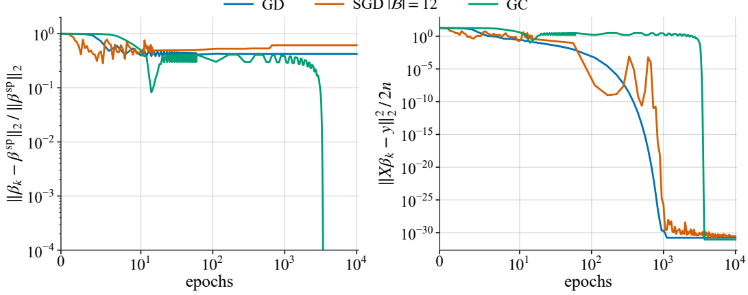
Figure 7. Sparse recovery in noiseless regression with cosine annealing from \gamma_{\max} = 0.35 to \gamma_{\min} = 0.05 . Left: normalized distance to the sparse teacher. Right: normalized training loss; GC recovers the sparse teacher substantially better than (S)GD.
