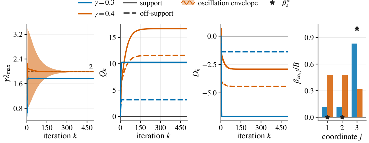
Figure 3. A diagonal linear network example case with control parameter B = 3.1 and learning rates \gamma = 0.3 and 0.4 . (Left) We plot the product of sharpness and step size. The smaller step size run converges below the EoS regime while larger learning rate oscillates. (Middle) In both cases, the Gain and the Drift accumulate comparatively (Lemma 2.5 and 2.6). (Right) We plot the predictor coefficient, recovering a sparser solution for the former run and denser for the latter.
