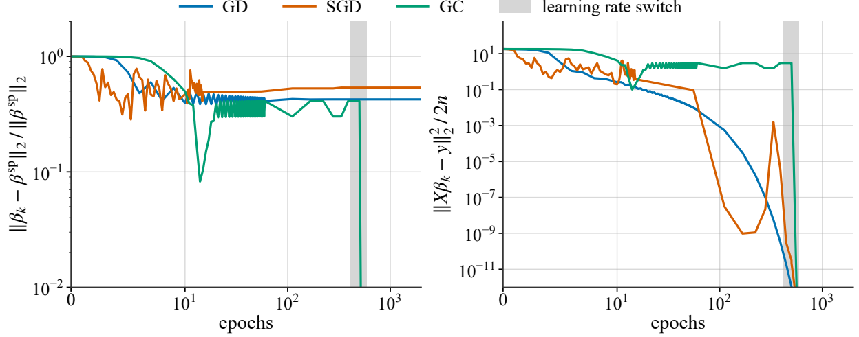
Figure 4. Sparse recovery for GD, SGD and GC on the noiseless sparse regression problem. ( Left ) Distance to the sparse teacher. Due to its implicit bias (Prop. 3.3), GC recovers a predictor substantially closer to the sparse teacher. ( Right ) Loss curve for the three methods. The learning rate switch is to allow GC to converge.
