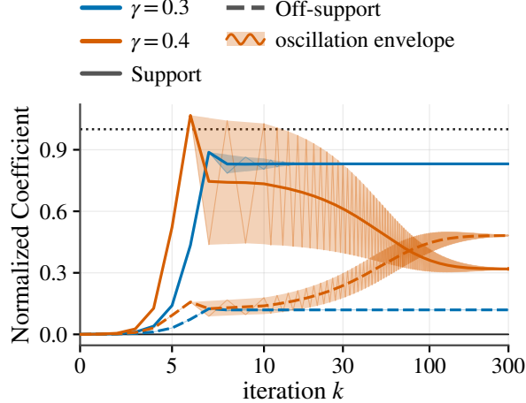
Figure 1. A diagonal linear network with learning rate \gamma = 0.3 and 0.4 to show the evolution of the predictor coefficient. The smaller step size does not reach the Edge of Stability regime, while the larger one does. We recover a sparser solution for the former.
