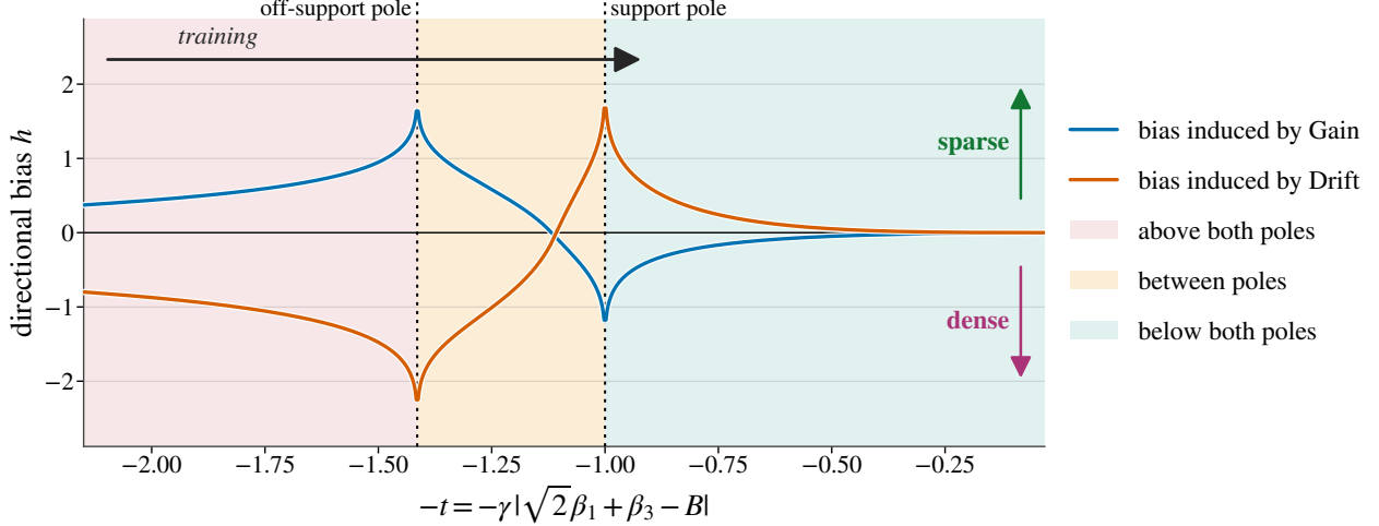
Figure 2. Alternating behavior of the Gain and the Drift. At initialization, the training starts from the left and proceeds to the right as the gradients shrink. The upper half of the plot indicates a sparsity promoting behavior, while the bottom half represents bias towards denser predictors. The two dotted lines represent the support and offsupport poles. See Table 1 for a summary.
