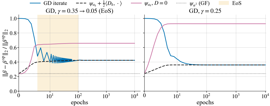
Figure 8. The Drift is necessary for sparse recovery. At every checkpoint k we minimise the implicit-bias potential over the interpolation manifold \mathcal{M} , using the Gain Q_k and Drift D_k accumulated so far, and plot the distance of that minimizer to the sparse teacher. With the Drift, \psi_{a_k} + \frac{1}{2}\langle D_k, \cdot \rangle (dashed) converges exactly to the GD iterate (blue), as predicted by Prop. 2.3. Keeping the same Gain but setting D = 0 (purple) selects a much denser interpolator. The gradient-flow potential \psi_{\alpha^2} (dotted, Q = D = 0 ) is shown for reference. GF recovers the sparsest solution. The shaded region marks the oscillatory phase ( \gamma_k S_k \geq 2 )
