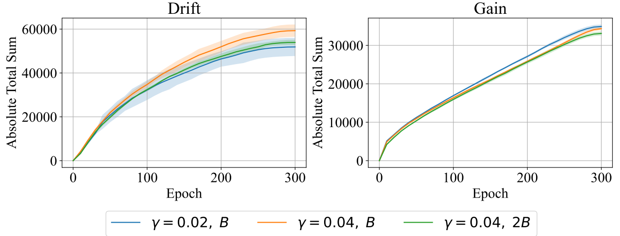
Figure 5. Accumulated Drift and Gain of all Query-Key pairs for a DeiT-Small trained on ImageNet with Muon, across three (batch size, learning rate) configurations. Both quantities grow substantially early in training, but Drift starts plateauing while Gain continues to accumulate throughout training.
