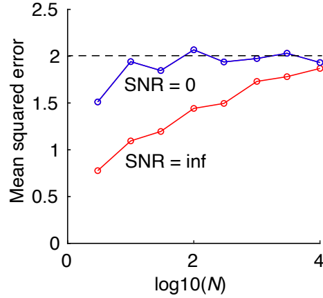
Figure 1: Numerical simulation of the generalization error of the nearest neighbor algorithm, for \alpha = 1 and SNR \mathcal{S} = \infty (red) and \mathcal{S} = 0 (blue). As input dimension N approaches infinity, generalization error in both cases approaches 2, consistent with our analytical derivation.
