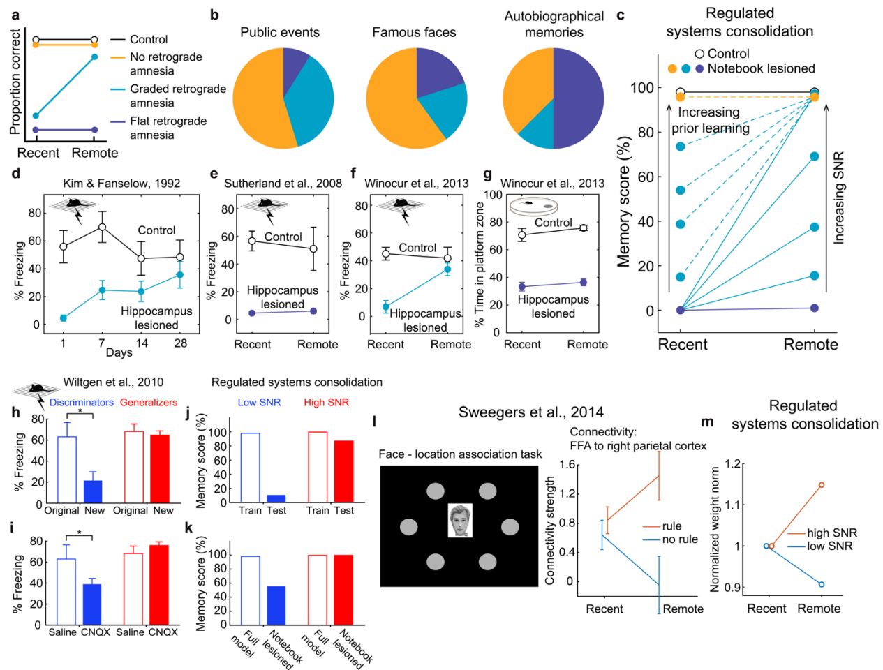
Fig. 3. Regulated systems consolidation mirrors memory research findings in both humans and rodents. (a) Schematic of retrograde amnesia curves. (b) Reports of retrograde amnesia in human patients with selective hippocampal damage show diverse dynamics. Figure adapted from Yonelinas et al., 2019 17 . (c) Regulated systems consolidation can reproduce the diversity of retrograde amnesia curves (see Methods for model details). (d, e) Lesioning hippocampus in rodents can produce both graded and flat retrograde amnesia. Figure adapted from Kim & Fanselow, 1992 57 , Sutherland et al., 2008 50 . Lesioning the hippocampus can result in graded (f) or flat (g) retrograde amnesia in the same animal performing different tasks (contextual fear conditioning and Morris water maze, respectively). Figure adapted from Winocur et al., 2013 51 . (h) Discriminators can differentiate the original fear-conditioning context with another similar but novel context, whereas generalizers show similar amount of fear response to both contexts. (i) Silencing the hippocampus in mice 15 days after contextual fear conditioning differentially impact fear memory of the original context, depending on whether the animal show time-dependent fear generalization. panels h and i are adapted from Wiltgen et al., 2010 58 . (j, k) Regulated systems consolidation can reproduce similar correlation between time-dependent generalization and reduced hippocampal dependence of memories. High SNR (1000) and low SNR (0.6) simulations based on analytical solutions are used to model the “generalizers” and “discriminator”. 2000 total epochs are simulated with N = P = 100 , notebook size M = 5000 , and learnrate = 0.005 . (l) Face-location association task with rules vs no rules show different time-dependent change in functional connectivity between cortical areas. Figure adapted from Sweegers et al., 2014 59 . (m) Regulated systems consolidation shows similar connectivity changes over time, as reflected in
