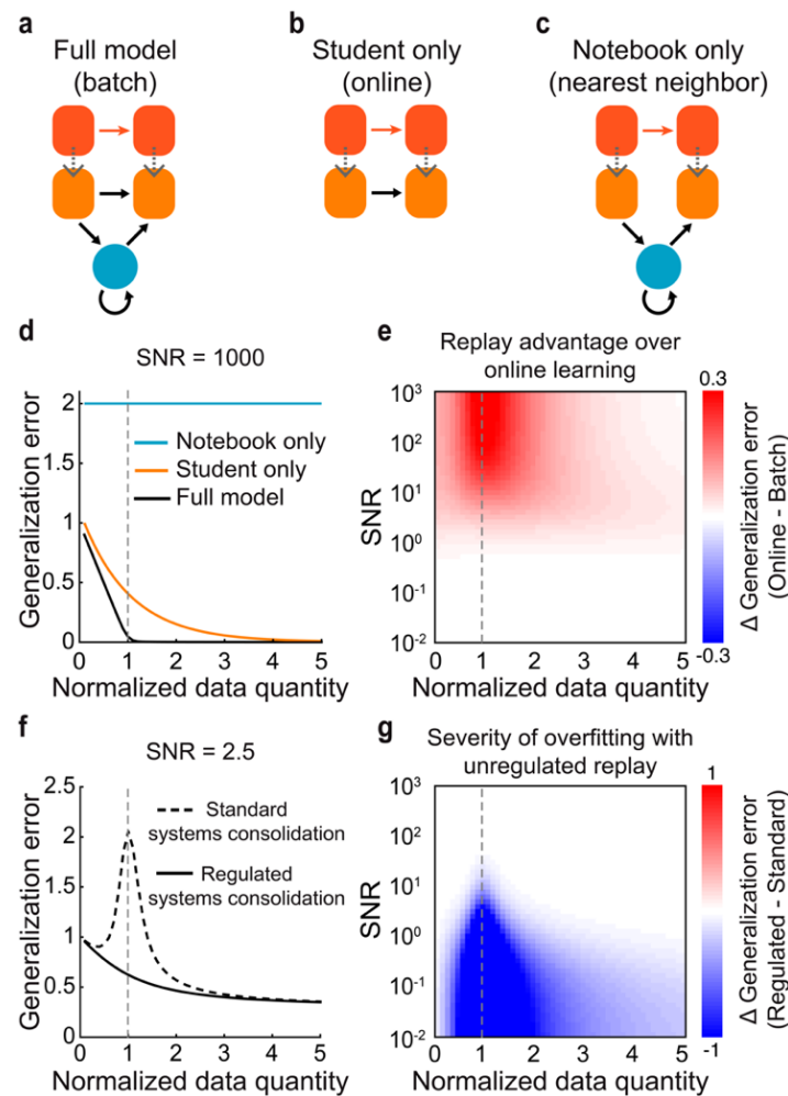
Fig. 4. Normative benefits of complementary learning systems for generalization. (a-c) Schematics illustrating learning systems that can use both the student and the notebook (a), only the student's weights (b), and only the notebook weights (c) for inference. In machine learning terminology, these systems implement batch learning, online learning, and nearest neighbor regression. (d) Generalization error as a function of normalized data quantity (or \alpha ( \alpha ), defined as \alpha = P/N ) for each learning system (SNR = 1000), dashed gray line indicates \alpha = 1 . (e) Advantage of regulated systems consolidation over optimal online learning as a function of SNR and normalized data quantity, measured by the difference in generalization error. (f) Generalization error as a function of normalized data quantity for the combined system, learning either through regulated systems consolidation or standard systems consolidation (SNR = 2.5). (g) Severity of overfitting, measured by the difference in generalization error between standard systems consolidation and regulated systems consolidation.
