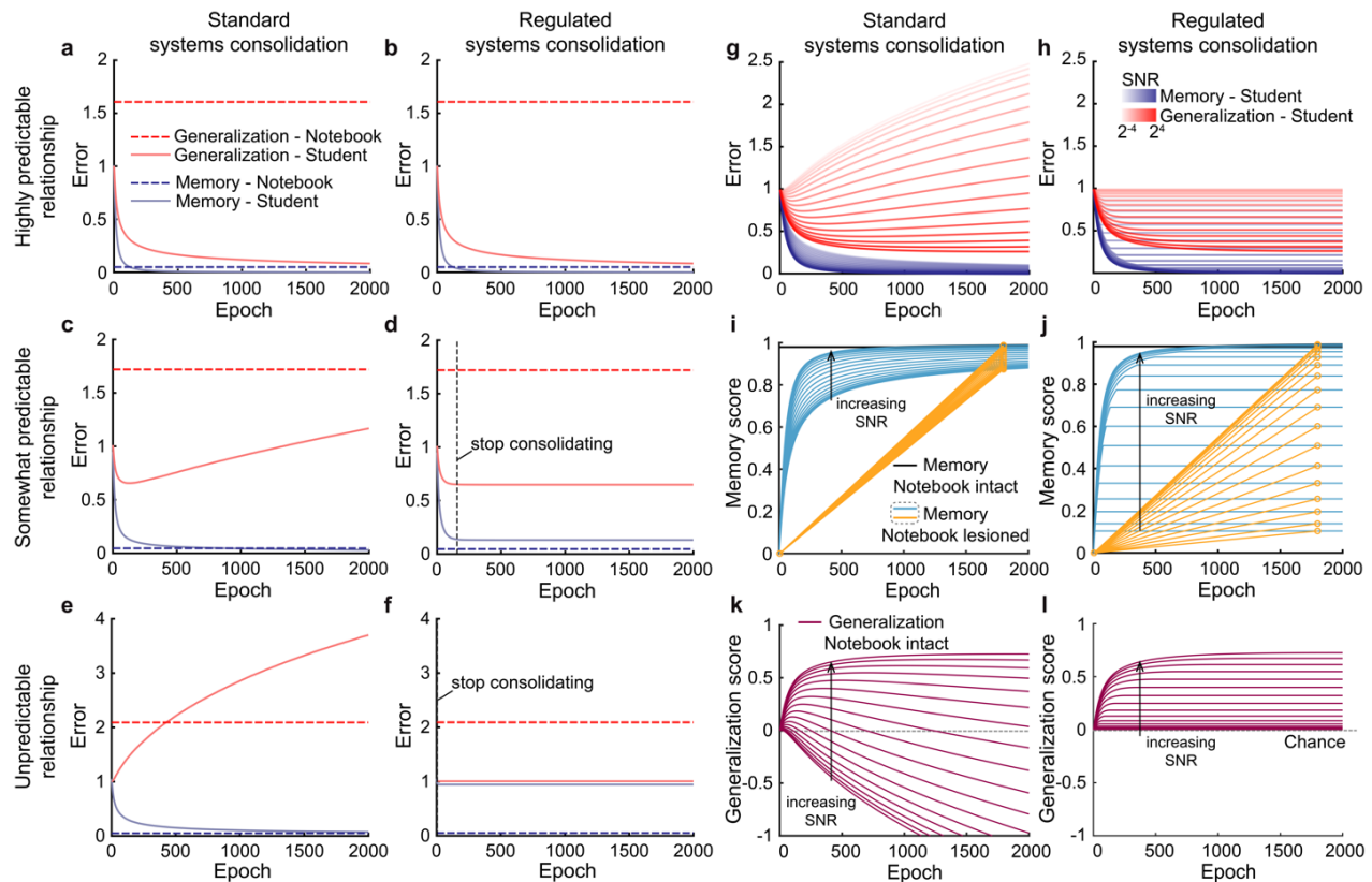
Fig. 2. The predictability of experience controls the dynamics of systems consolidation. (a-h) Dynamics of student generalization error, student memorization error, notebook generalization error, and notebook memorization error when optimizing for student memorization (a, c, e, g) or generalization (b, d, f, h) performance. The student's input dimension N = 100 , and the number of patterns stored in the notebook P = 100 (all encoded at epoch = 1; epochs in the x-axis correspond to the time passage during systems consolidation). Notebook contains M = 2000 units, with a sparsity a = 0.05 . During each epoch, 100 patterns are randomly sampled from the P stored patterns for reactivation and training the student. The student's learning rate is 0.015. Teachers differed in their levels of predictability (a, b: SNR = infinity; c, d: SNR = 4; e, f: SNR = 0.05; g, h: SNR ranges from 2^{-4} to 2^4 ). (i-l) Memorization and generalization scores for the integrated student-notebook system as a function of time and SNR, when optimized for student memorization (i, k) or generalization (j, l). Memory and generalization scores are translated from respective error values by \text{Score} = (E_0 - E_t)/E_0 , E_0 and E_t are the generalization or memory errors before training starts and at epoch = t , respectively. Effect of notebook lesion on memory performance (cyan and orange lines, orange lines are simply the two-point version of the cyan lines) depended on optimization objective and time (i, j).
