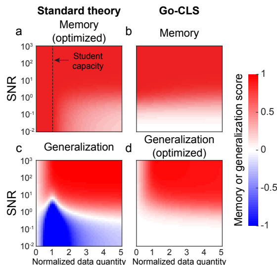
Figure 2: Heatmaps of student memorization performance (a, b) and generalization performance (c, d) as a function of SNR and \alpha , when optimized for student memorization (a, c) or generalization (b, d).
