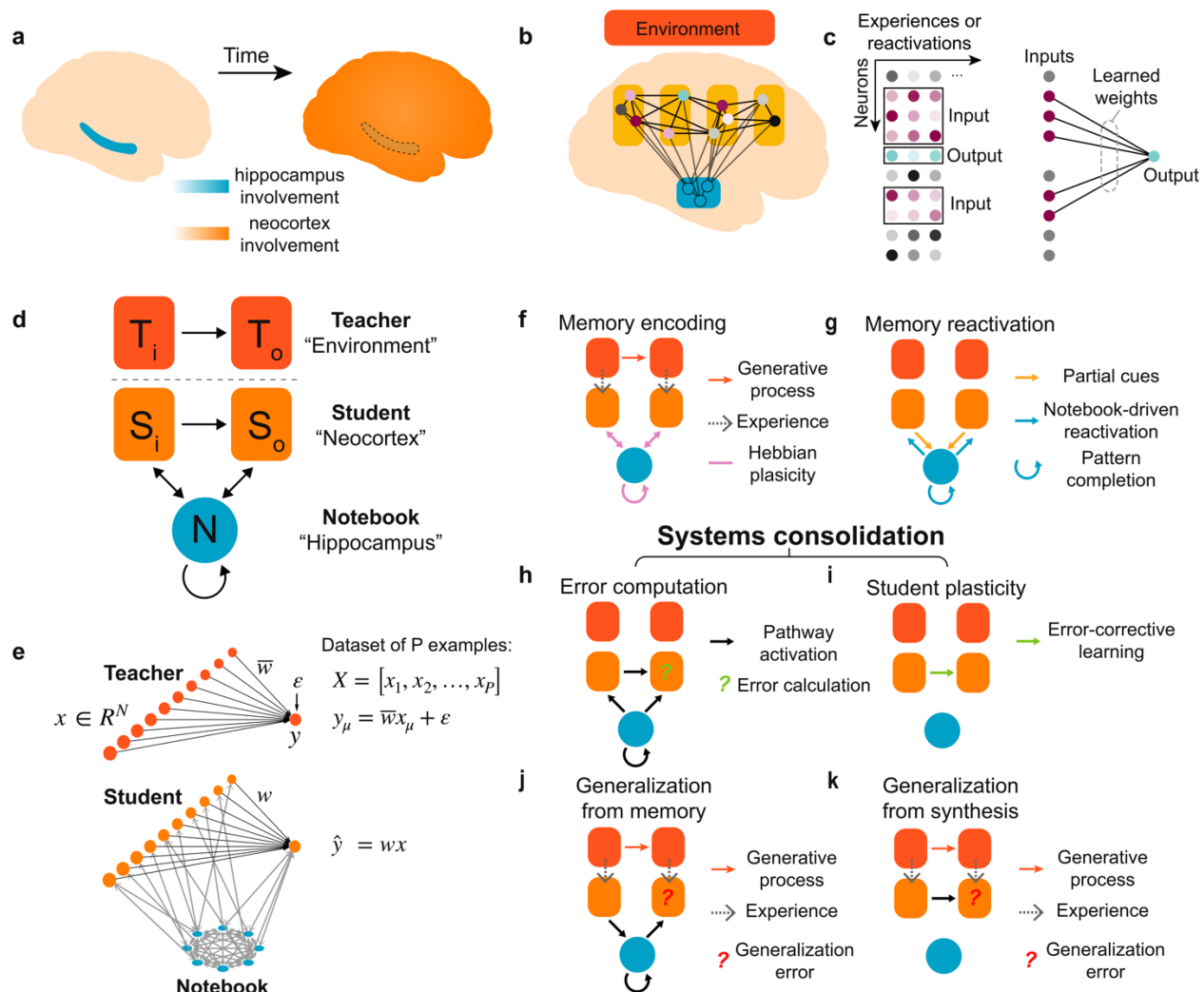
Fig. 1. Neural network model of systems consolidation. (a) The standard theory of systems consolidation. (b, c) Our theoretical framework assumes that neocortex extracts and encodes environmental relationships within the weights between distributed neocortical neurons in a process mediated by hippocampal reactivations. (d) Cartoon of the teacher-student-notebook formalism; subscripts "i" and "o" refer to input and output layers. (e) Core neural network model architecture (see Methods for details). (f-k) Stages of learning and inferences in the model.
