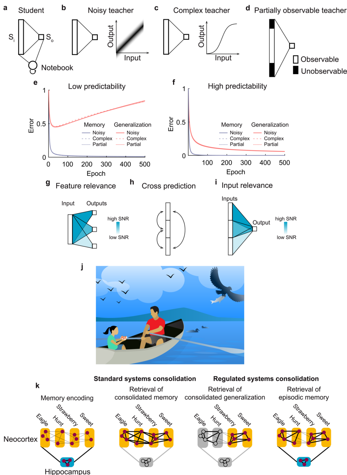
Fig. 5. Many forms of unpredictability demand regulated systems consolidation. (a) The student-notebook learning system. (b-d) Example teachers with unpredictable elements. (b) A teacher that linearly transforms inputs into noisy outputs. (c) A teacher that applies a nonlinear activation function at the output unit. (d) A teacher that only partially reveals the relevant inputs to the learning system. (e, f) Varying predictability within the three different teachers all lead to quantitatively similar learning dynamics
