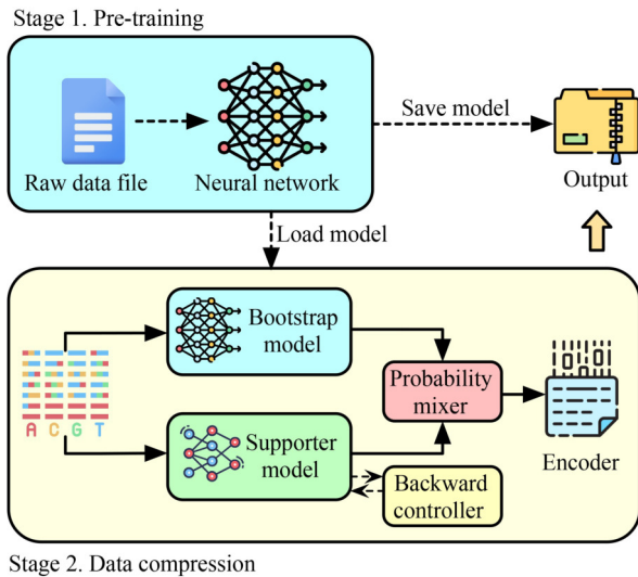
Fig. 3 The compression process of the semi-adaptive methods
