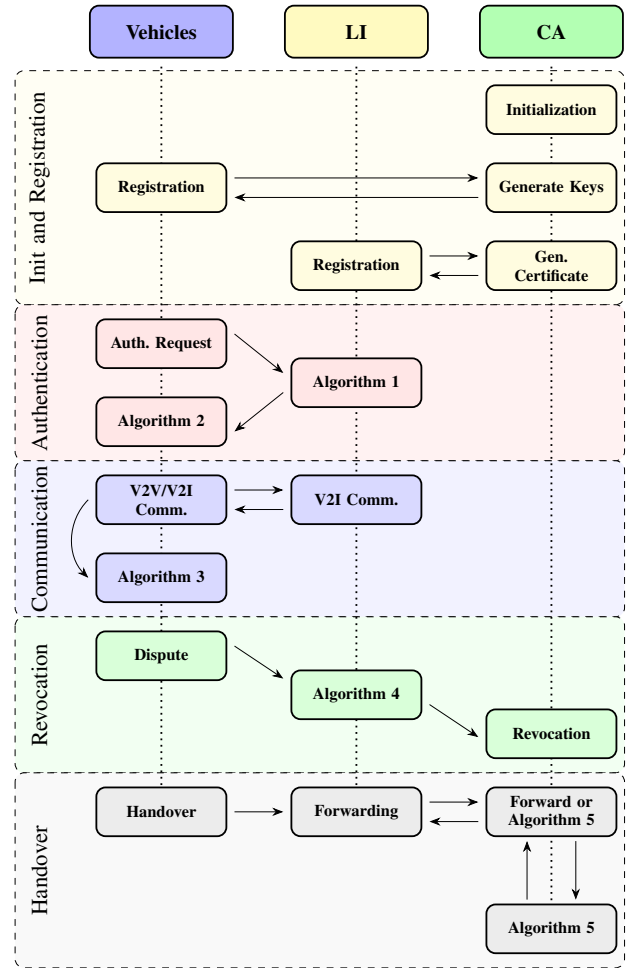
FIGURE 3: Protocols phases denoting the parties involved and the algorithms executed.
