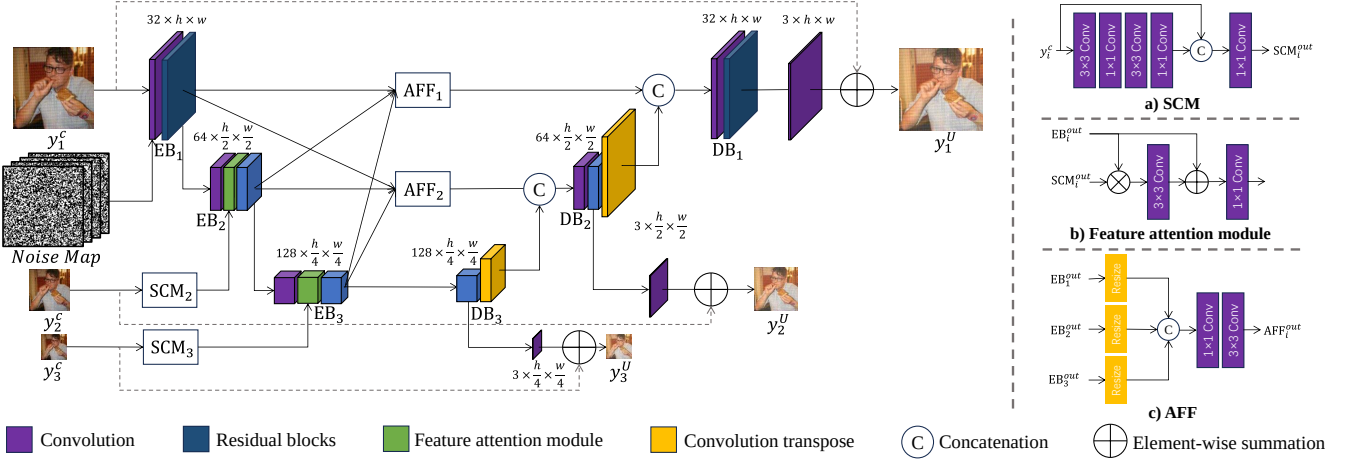
Figure 5: The overall framework of the modified MIMO-UNet. It consists of an encoder that receives downsampled noise images at different scales and a Gaussian noise map sampled from a random normal distribution as input. The Shallow Convolutional Module (SCM) initially extracts features, followed by an Encoder Block (EB) containing a Feature Attention Module (FAM) that progressively extracts multi-level features. Between the encoder and decoder, an Asymmetric Feature Fusion (AFF) module is introduced to effectively fuse features at different scales. During the decoding phase, the network uses a single decoder to generate multiple deburred images at different scales via the Decoder Block (DB). On the right side of the figure, from top to bottom, are the structures of the SCM, Feature Attention Module and AFF.
