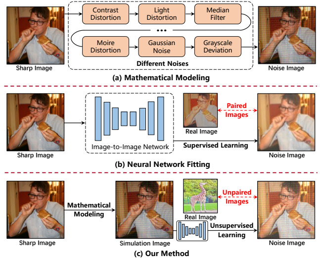
Figure 1: Overview of traditional noise approximation strategies and proposed Simulation-to-Real. (a) Mathematical modeling-based noise approximation. (b) Supervised neural fitting via paired images. (c) Our method: transforming sharp images to a certain noise domain, then mapping them unsupervised to an unknown domain, achieving more realistic noise approximation.
