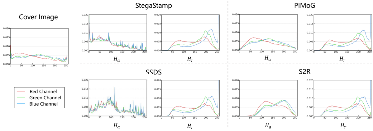
Figure 6: Comparison between approximate noise images under different schemes. Where H_r represents the histogram of real SC Image, and H_a represents the histogram of approximate noise Images. For all histograms, the horizontal axis represents pixel intensity ranging from 0 to 255, while the vertical axis represents the average normalized frequency ranging from 0 to 1.
