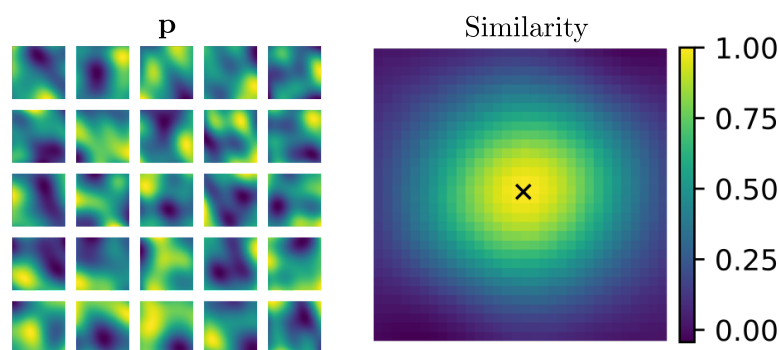
Figure 5: Similarity-preserving spatial representations. The left-hand side shows example ratemaps of a model whose eigenvalues are sampled from a normal distribution, such that the similarity function is approximately Gaussian. The resulting similarity, relative to the origin, is shown on the right-hand side.
