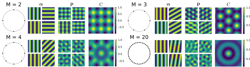
Figure 2: Example plane waves ( \alpha ) and corresponding representations ( \mathbf{p} ) alongside the similarity function ( C ) relative to the origin (black cross) for representations whose eigenvalues form sets of roots of unity, with symmetries M on a single ring. For each eigenvalue (imaginary part indicated by black dot), the corresponding conjugate eigenvalue is also shown. Representations were formed using generators with a single set root-of-unity solution with varying M , a random orthogonal matrix R , and \mathbf{p}_0 = R^T \mathbf{1} .
