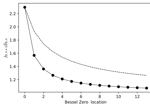
Figure 4: Ratio of subsequent zeros of the Bessel function J_0 (large dots), alongside a cumulative average (dashed line).
