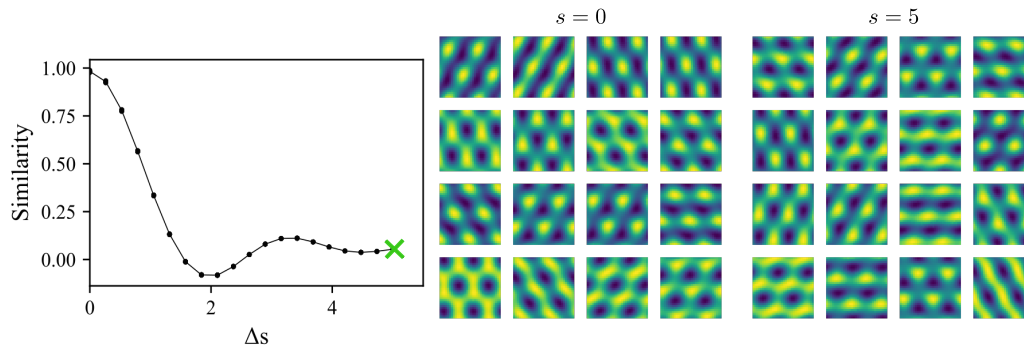
Figure 3: Between-context similarity as a function of context separation. Also inset are example ratemaps for two distant context values ( s = 0 , s = 5 ) corresponding to \Delta s = 5 . Representations were formed using generators with 10 identical root-of-unity solutions with M = 3 , a random orthogonal matrix R , and \mathbf{p}_0 = R^T \mathbf{1} .
