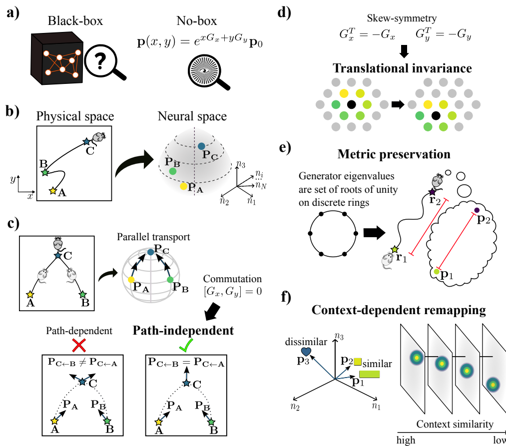
Figure 1: Conceptual overview of the proposed framework and results. a) Deep learning models are “black-boxes” that learn spatial representations, but the underlying principles are obscured by the complexities of architecture, training, and objective functions. The exponential map model is a transparent “no-box” alternative, using generator matrices ( G_x, G_y ) to construct a representation \mathbf{p}(x, y) . b) A neural population vector, which captures the activity of the entire neural ensemble, is assigned to every location, mapping physical space to a neural representational space. c) Path Invariance: Path integration can be viewed as a form of parallel transport, where a vector representing the neural representation is moved along a trajectory in a high-dimensional state space. Traversing a curved manifold can induce a net transformation in the vector at a point that is dependent on the traversal route. By imposing simple, interpretable algebraic constraints on the model’s generators, we can directly enforce fundamental properties. Path invariance is guaranteed if the generators commute. d) Translational Invariance: Making the generator matrices skew-symmetric ( G^T = -G ) imposes several biologically-relevant properties on the representation. First, it ensures that spatial relationships are consistently maintained across locations (translational invariance). Second, skew-symmetric generators produce orthogonal representations, meaning the population vector \mathbf{p}(x, y) maintains a constant norm across the entire space. e) Metric Preservation: Preserving the geometry of flat space requires the generator eigenvalues to form sets of roots of unity on discrete rings in frequency space, which, for certain symmetry orders gives rise to grid-like patterns. f) Remapping: Generalizing the framework to non-spatial inputs, like a context signal, allows the model to produce distinct spatial maps for different contexts, mimicking remapping.
