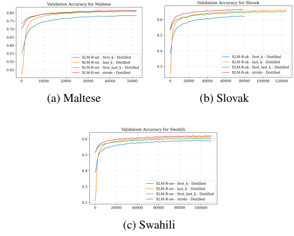
Figure 6: Validation accuracy for various initialization strategies for XLM-R.
