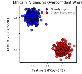
(c) Contrastive Embedding Separation
