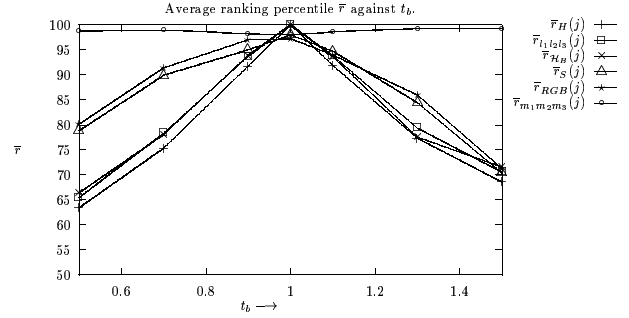
Figure 2: The discriminative power plotted against the change \beta in the color composition of the illumination spectrum.
