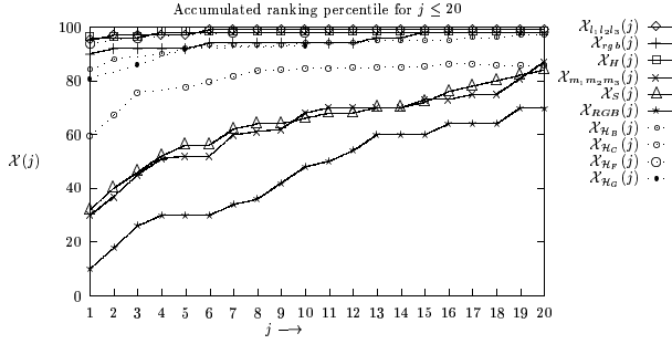
Figure 1: The discriminative power: the cumulative percentile \mathcal{X} for H , l_1 l_2 l_3 , rgb , S , m_1 m_2 m_3 , RGB , \mathcal{H}_B , \mathcal{H}_C , \mathcal{H}_F and \mathcal{H}_G is given by \mathcal{X}_H , \mathcal{X}_{l_1 l_2 l_3} , \mathcal{X}_{c_1 c_2 c_3} , \mathcal{X}_{rgb} , \mathcal{X}_S , \mathcal{X}_{m_1 m_2 m_3} , \mathcal{X}_{RGB} , \mathcal{X}_{\mathcal{H}_B} , \mathcal{X}_{\mathcal{H}_C} , \mathcal{X}_{\mathcal{H}_F} and \mathcal{X}_{\mathcal{H}_G} respectively.
