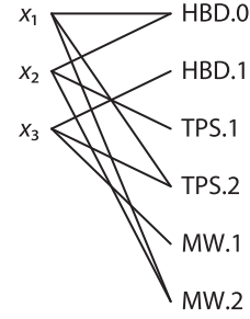
Fig. 2 The bipartite graph corresponding to the upper context.
