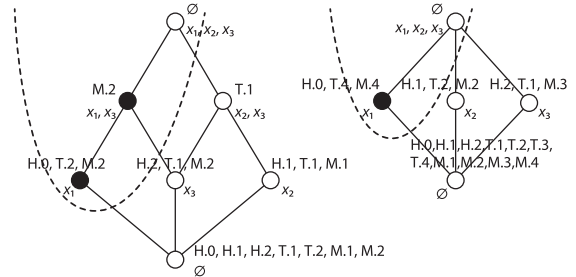
Fig. 5 Concept lattices constructed from contexts \mathcal{B}^1(\tau) (left) and \mathcal{B}^2(\tau) (right) in Table 5. The tuple y is consistent with concepts denoted by black dots.
