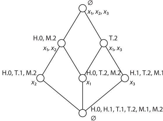
Fig. 3 A concept lattice constructed from the context in Table 2. Feature names HBD, TPS, and MW are abbreviated as H, T, and M, respectively.
