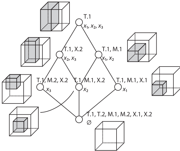
Fig. 4 The concept lattice \mathcal{B}^1(\tau) with its geometric interpretation.
