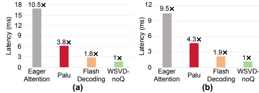
Figure 5: Latency evaluation and normalized latency on: (a) RTX 4090 and (b) RTX 5090.
